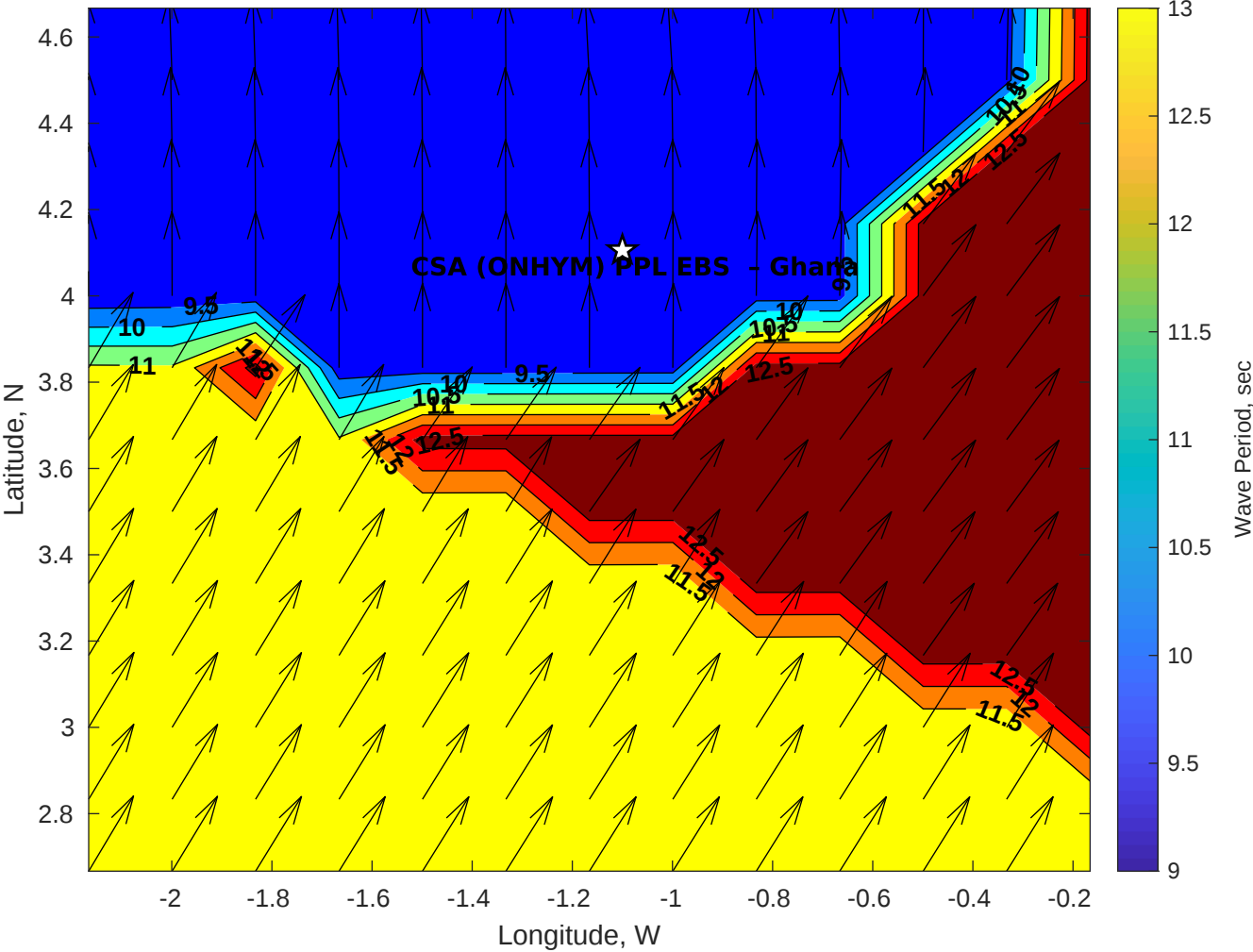
GFS Wave Period (sec) for CSA (ONHYM) PPL EBS - Ghana at 27-Dec-2025 09:00:00
