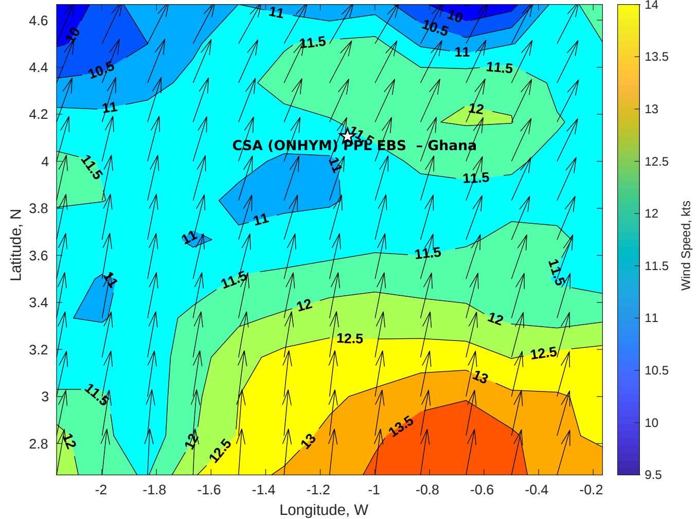
GFS Winds (kts) for CSA (ONHYM) PPL EBS - Ghana at 27-Dec-2025 09:00:00
