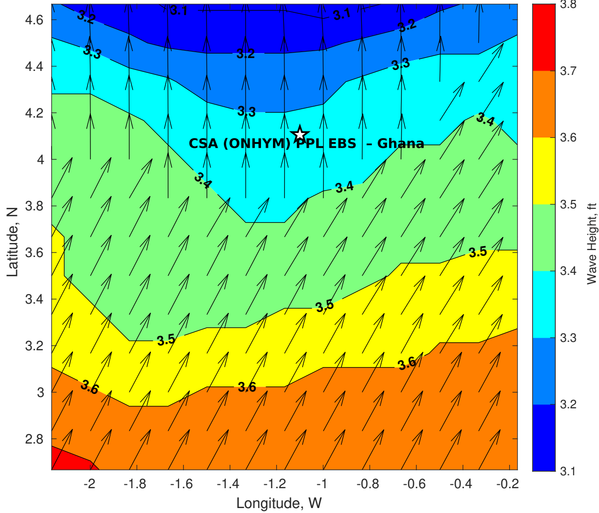
GFS Wave Height (ft) for CSA (ONHYM) PPL EBS - Ghana at 27-Dec-2025 09:00:00
