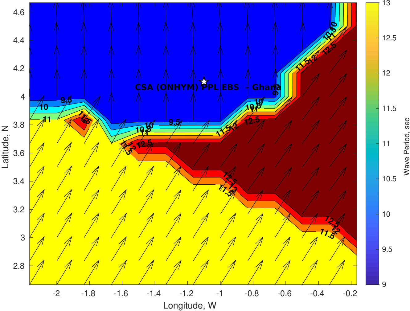
GFS Wave Period (sec) for CSA (ONHYM) PPL EBS - Ghana at 27-Dec-2025 09:00:00
