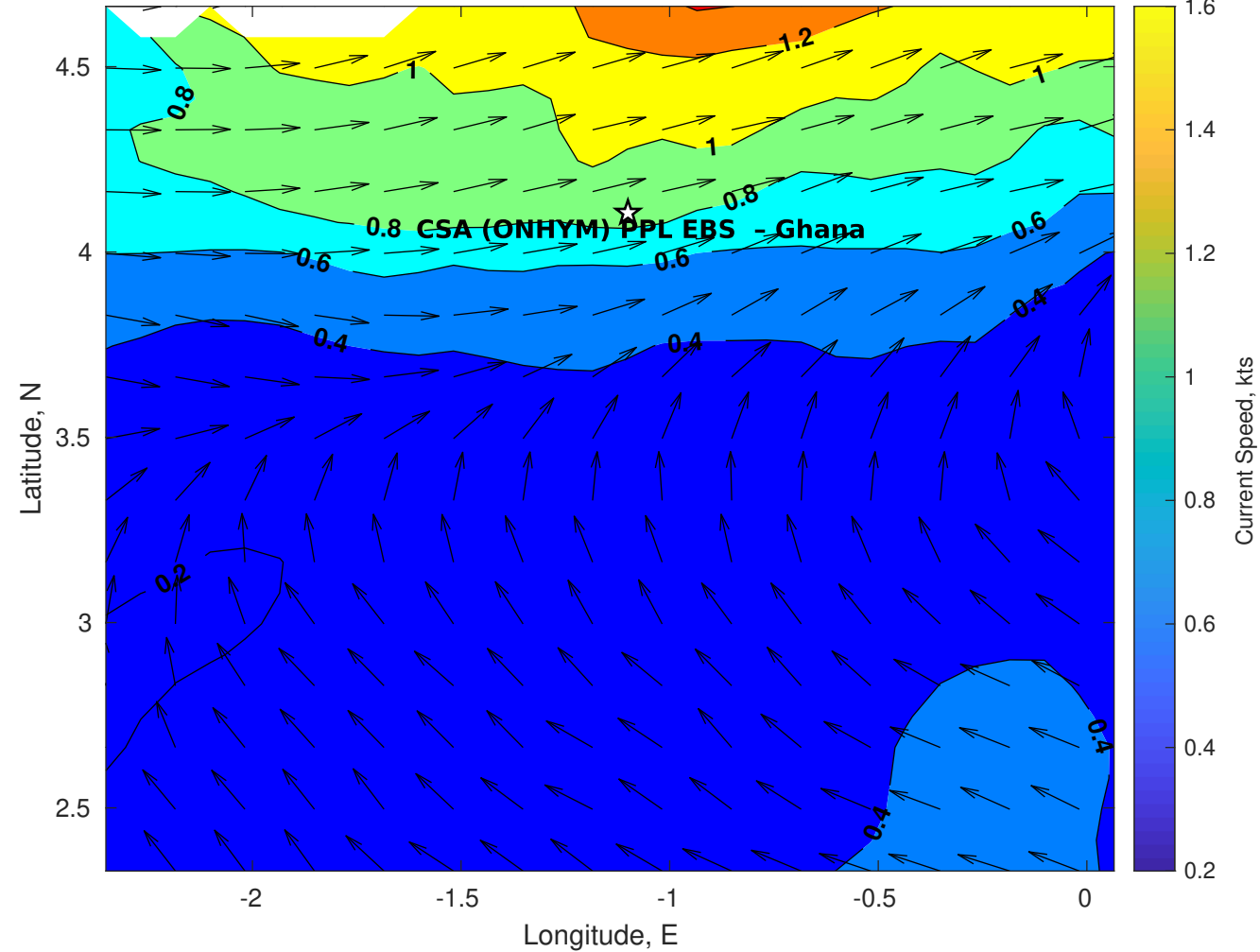
Surface Currents for CSA (ONHYM) PPL EBS - Ghana at 26-Dec-2025 00:00:00
