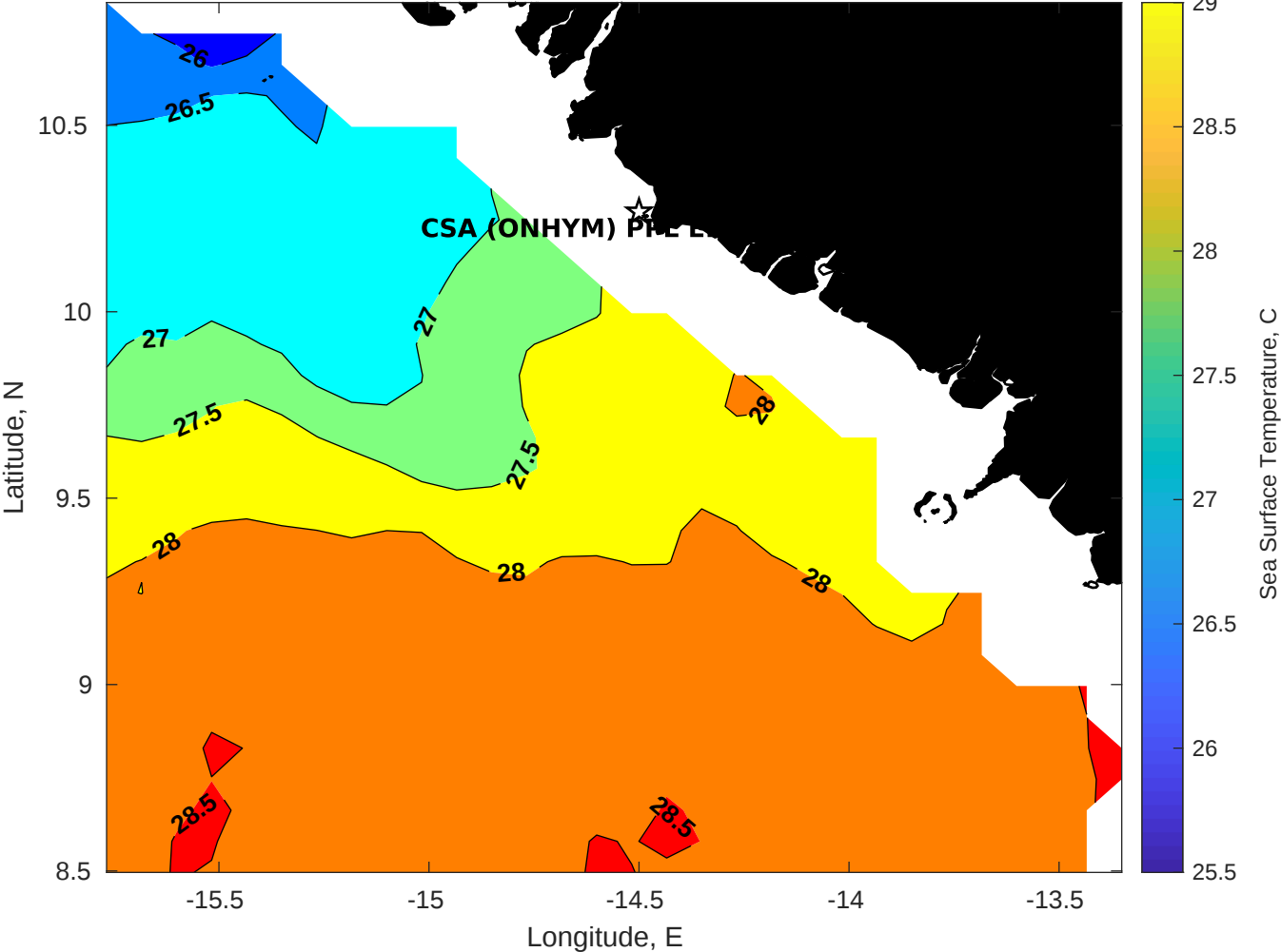
SST for CSA (ONHYM) PPL EBS - Guinea at 26-Dec-2025 00:00:00
