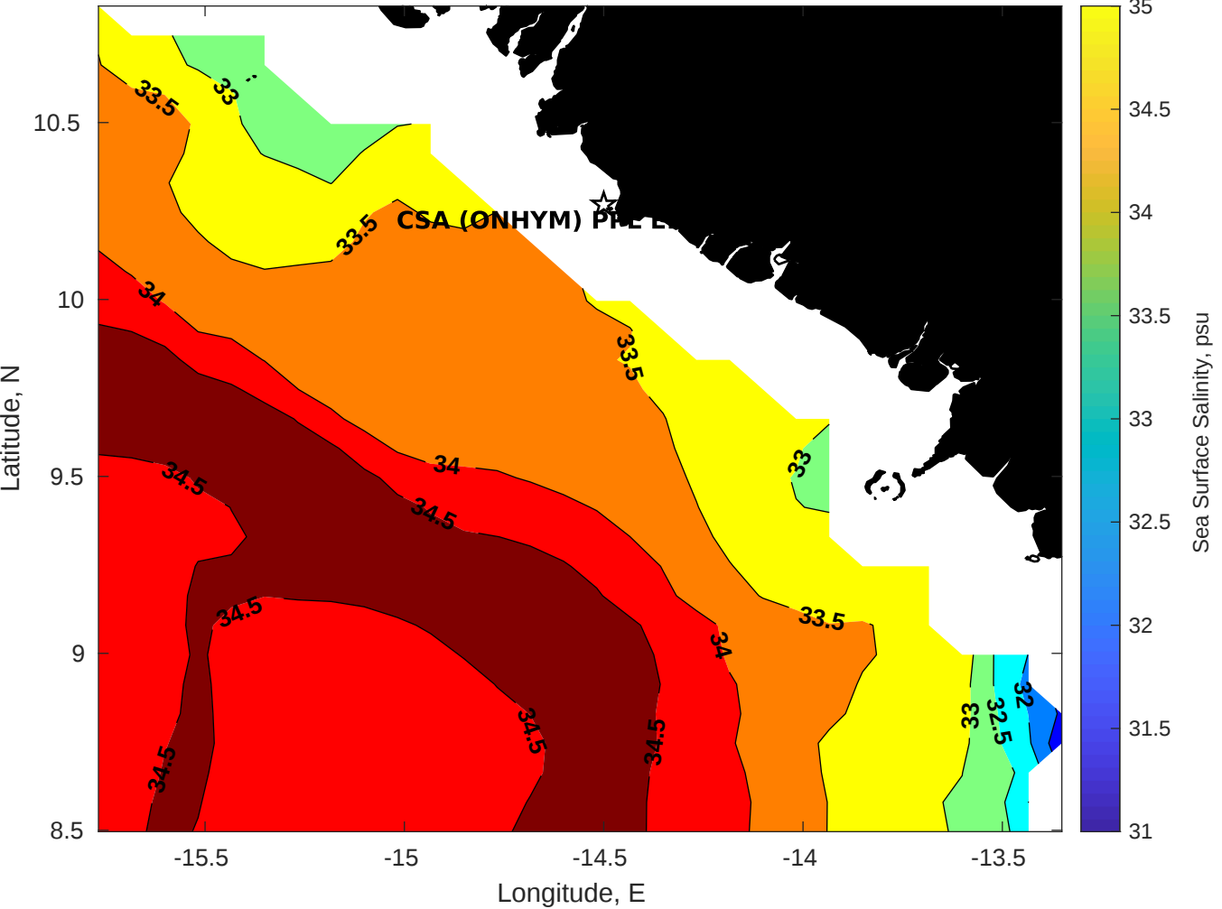
Surface Salinity for CSA (ONHYM) PPL EBS - Guinea at 26-Dec-2025 00:00:00
