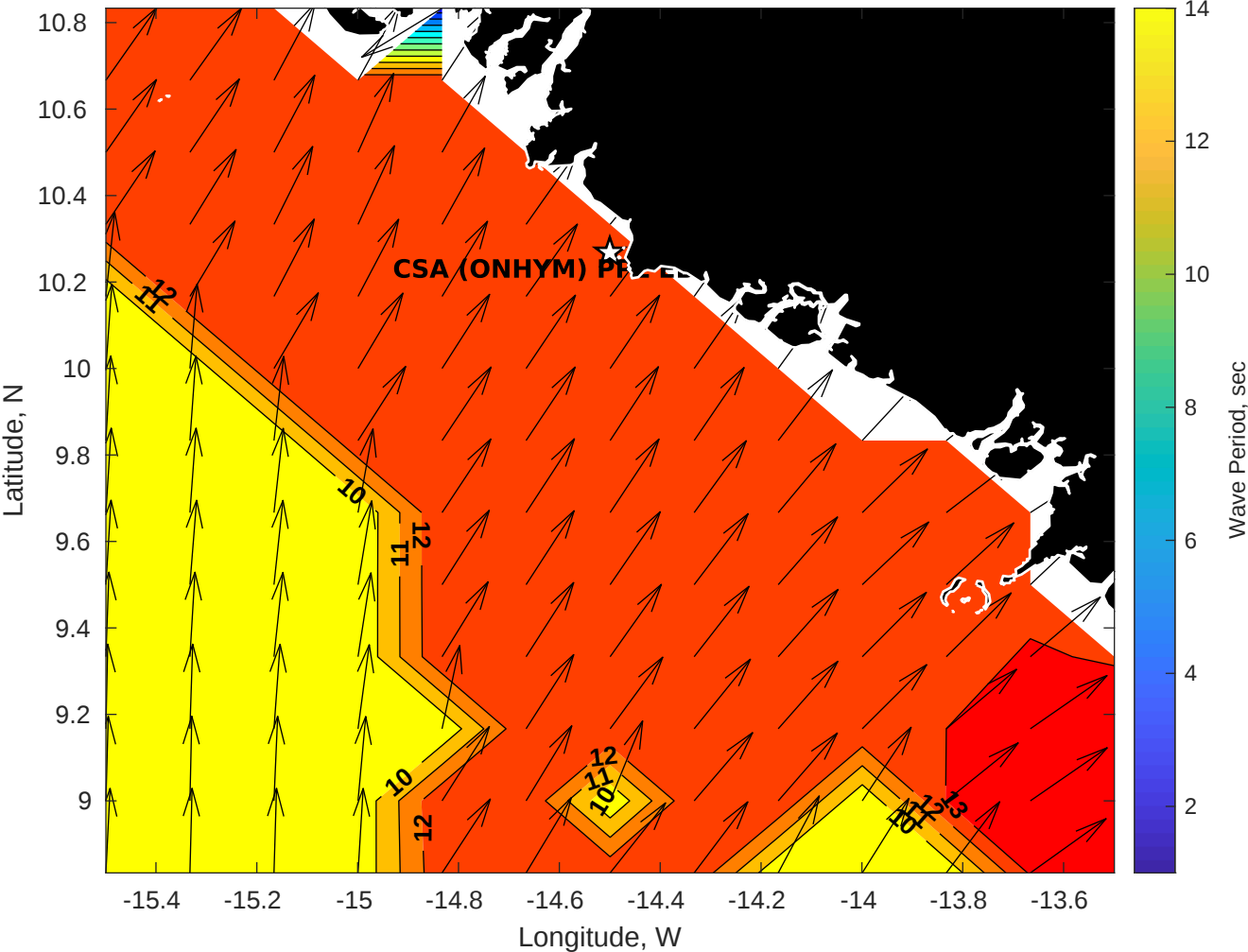
GFS Wave Period (sec) for CSA (ONHYM) PPL EBS - Guinea at 27-Dec-2025 09:00:00
