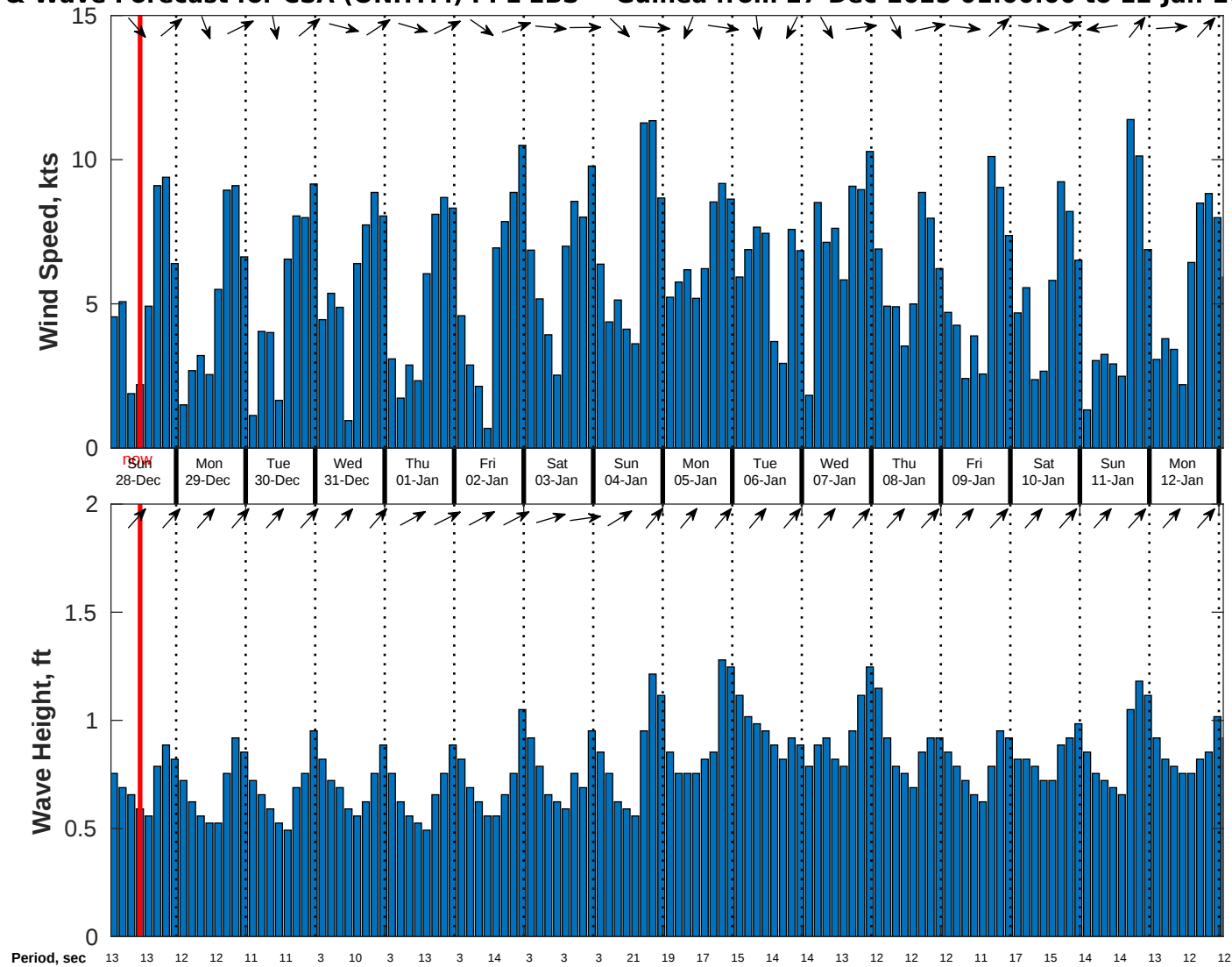
Wind & Wave Forecast for CSA (ONHYM) PPL EBS - Guinea from 27-Dec-2025 01:00:00 to 12-Jan-2026 01:00:00
