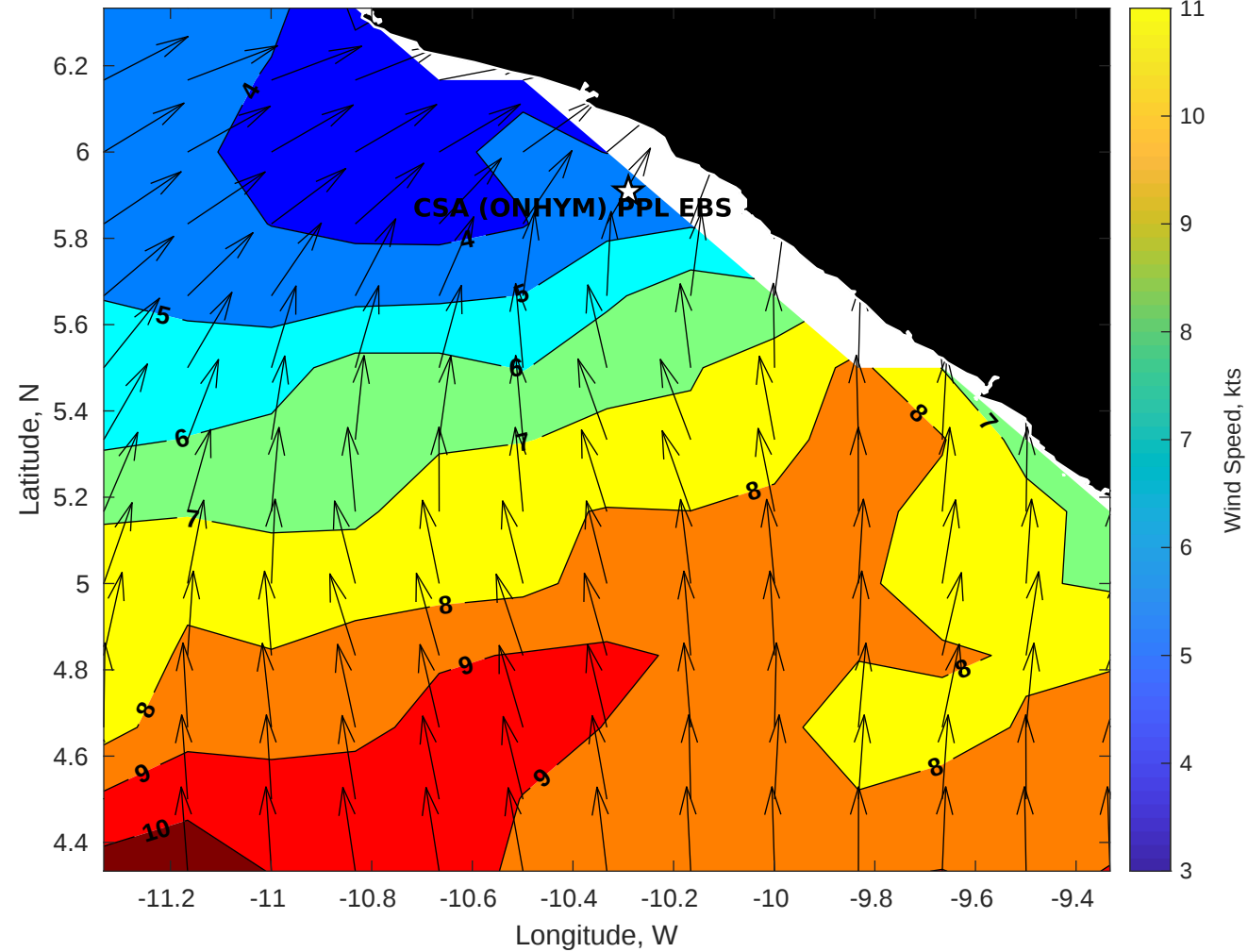
GFS Winds (kts) for CSA (ONHYM) PPL EBS - Liberia at 27-Dec-2025 09:00:00
