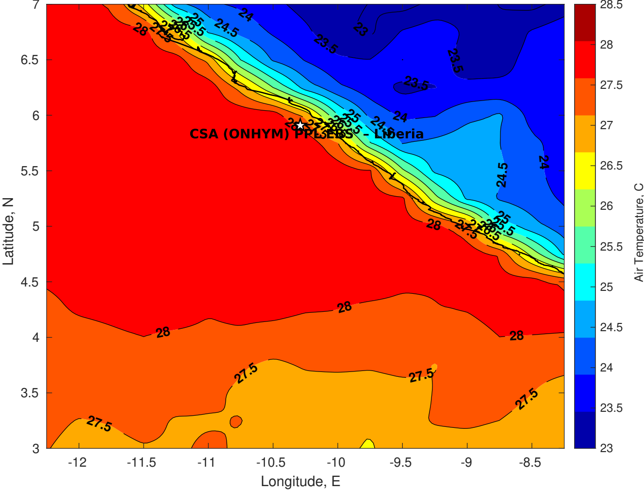
Air Temperature (C) for CSA (ONHYM) PPL EBS - Liberia at 27-Dec-2025
