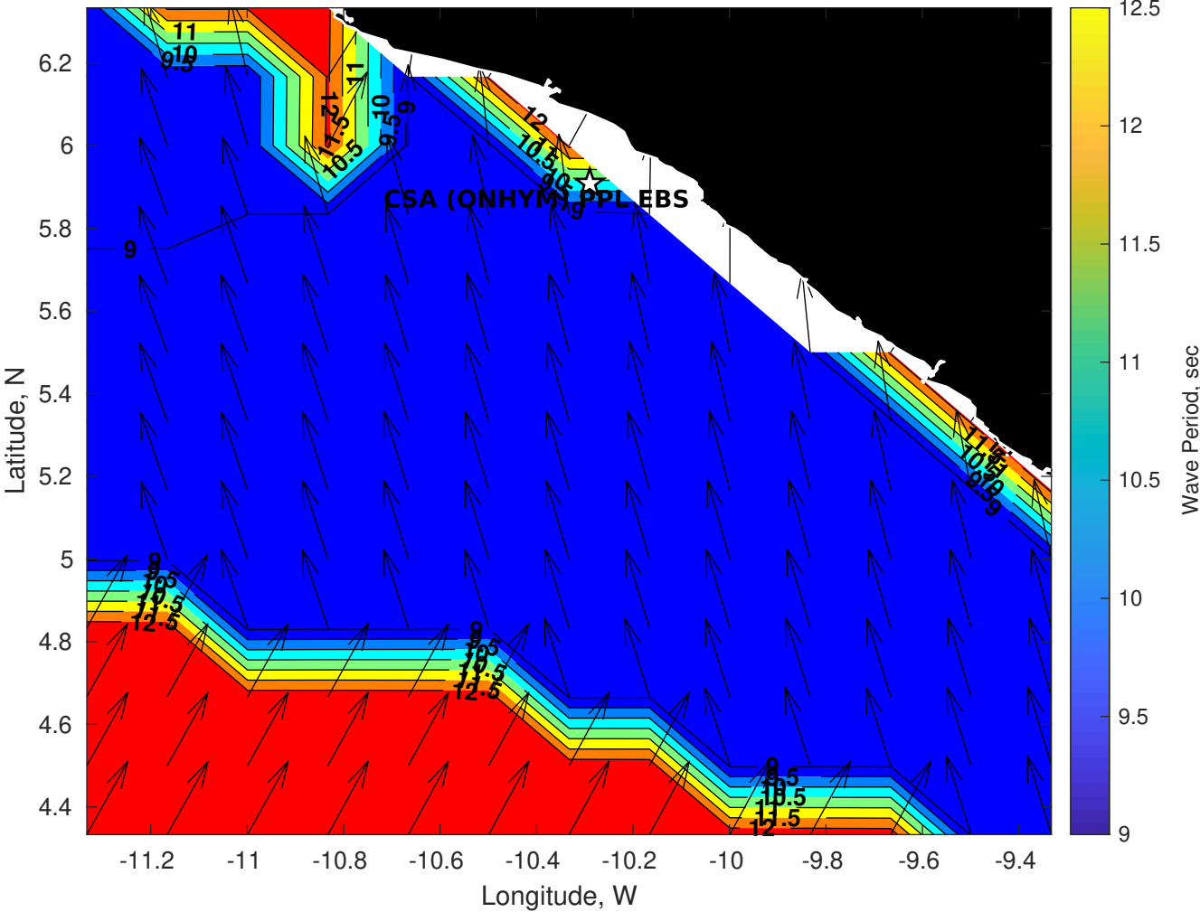
GFS Wave Period (sec) for CSA (ONHYM) PPL EBS - Liberia at 27-Dec-2025 09:00:00
