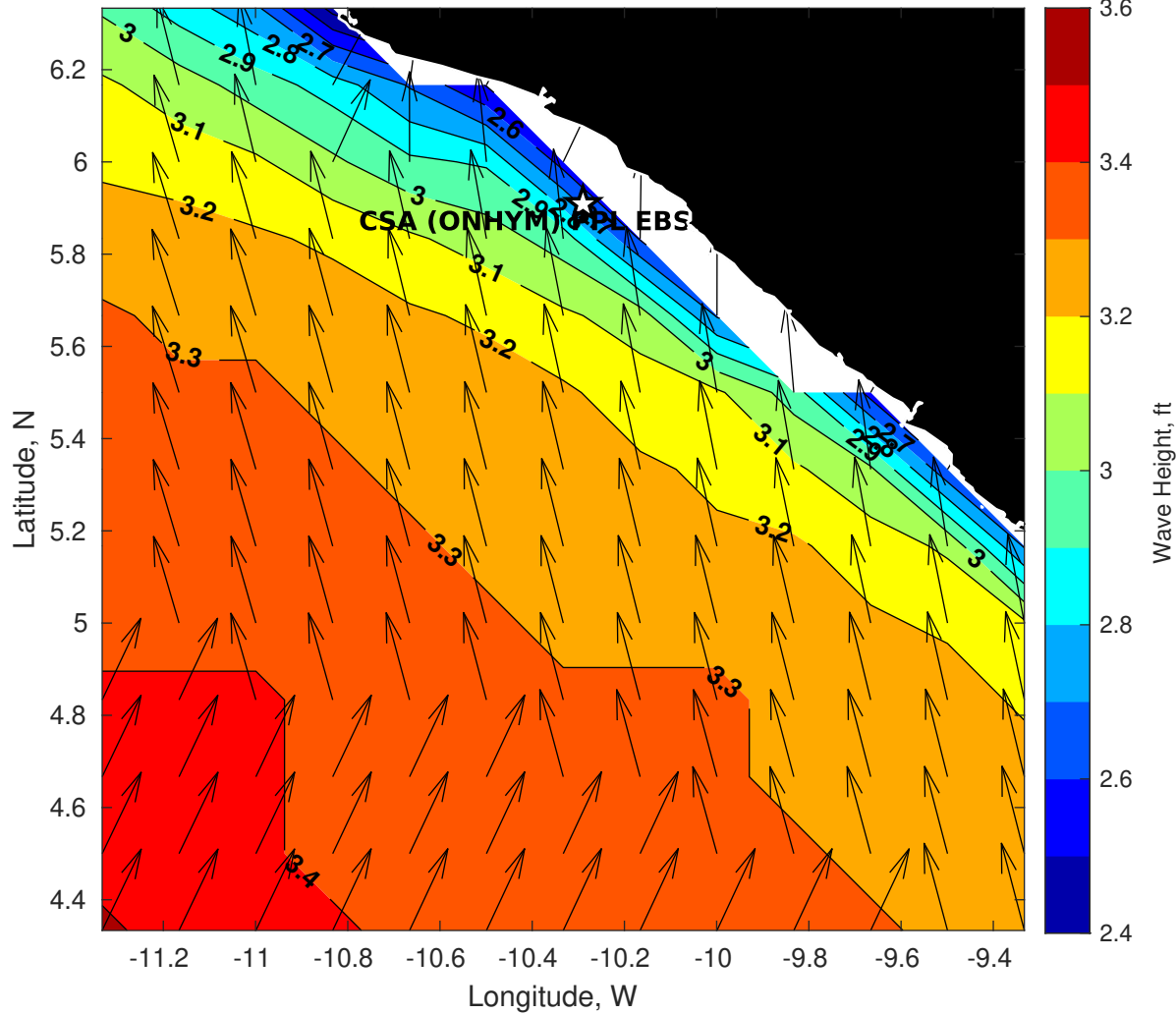
GFS Wave Height (ft) for CSA (ONHYM) PPL EBS - Liberia at 27-Dec-2025 09:00:00
