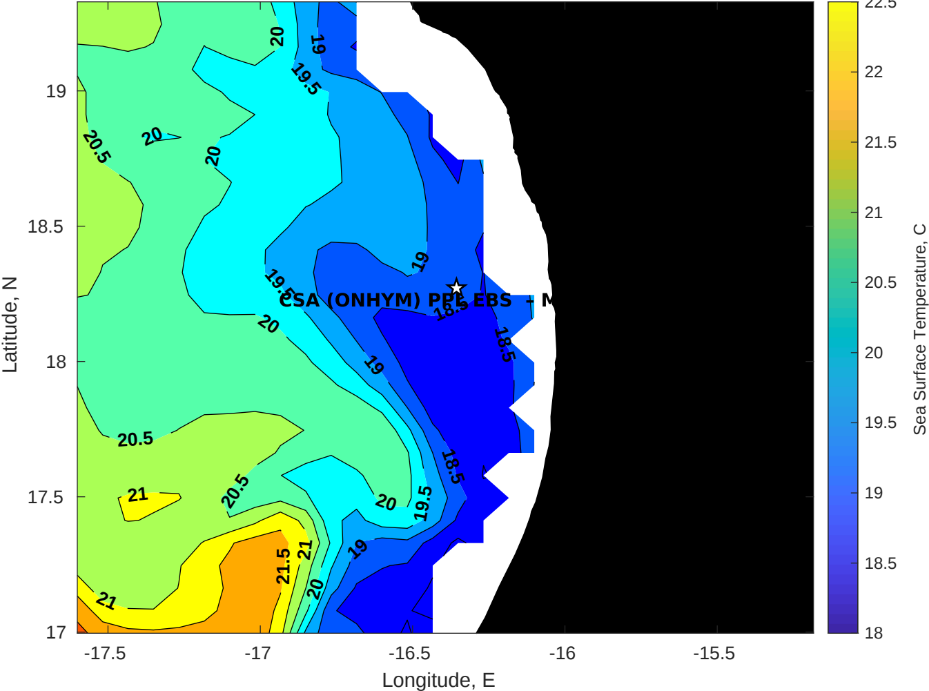
SST for CSA (ONHYM) PPL EBS - Mauritania at 26-Dec-2025 00:00:00
