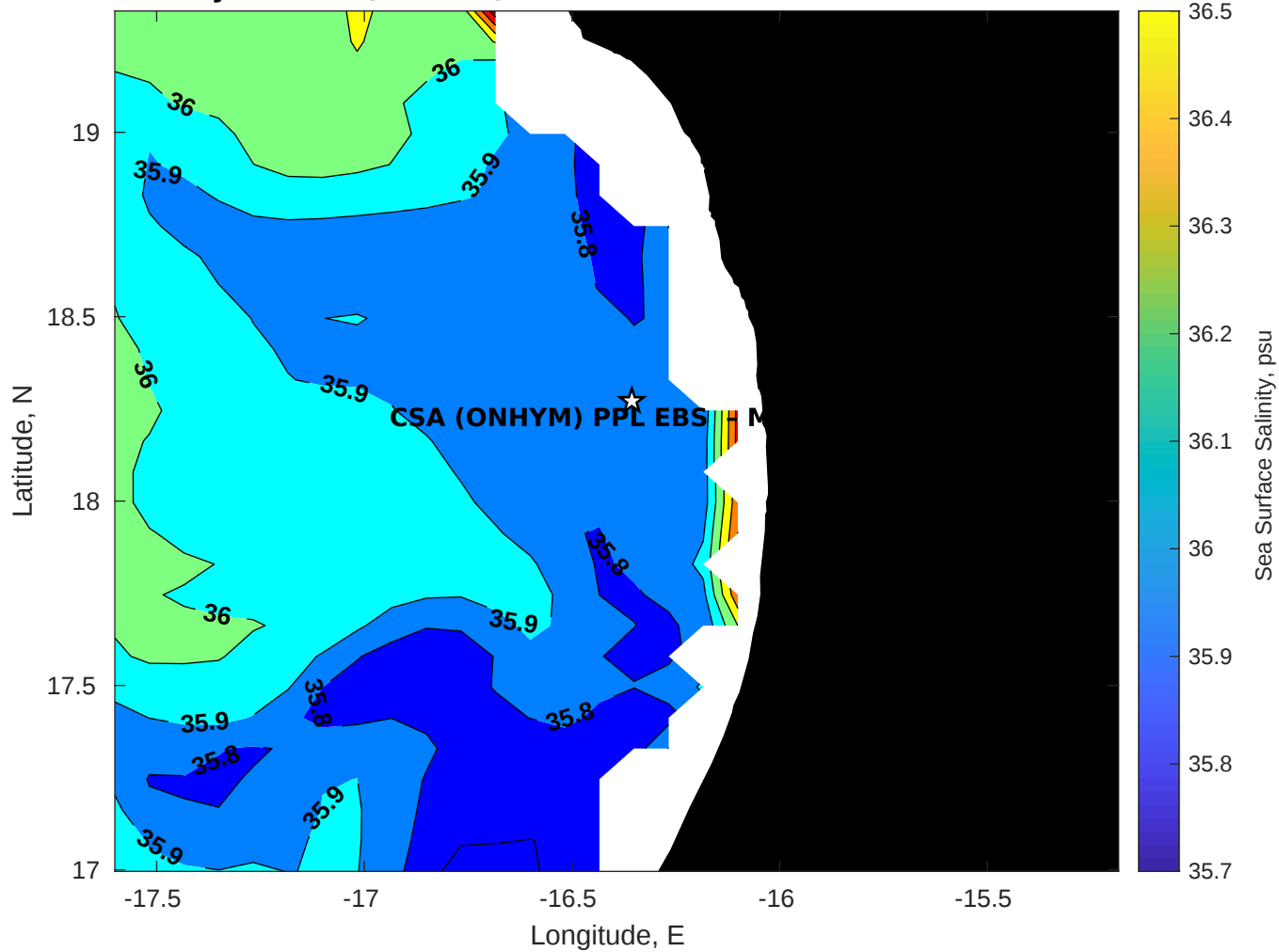
Surface Salinity for CSA (ONHYM) PPL EBS - Mauritania at 26-Dec-2025 00:00:00
