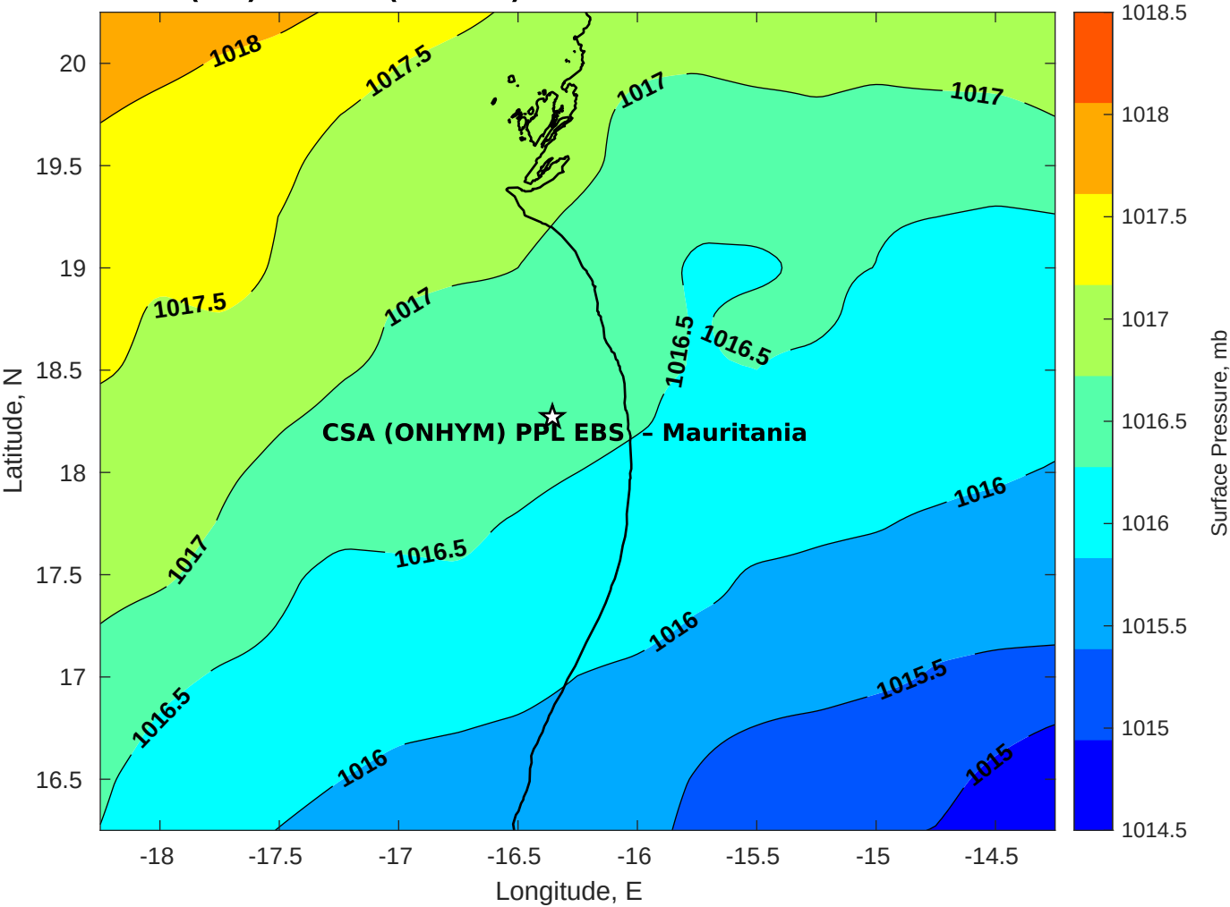
Surface Pressure (mb) for CSA (ONHYM) PPL EBS - Mauritania at 27-Dec-2025 00:00:00
