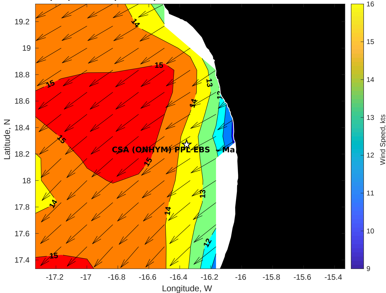
GFS Winds (kts) for CSA (ONHYM) PPL EBS - Mauritania at 27-Dec-2025 09:00:00
