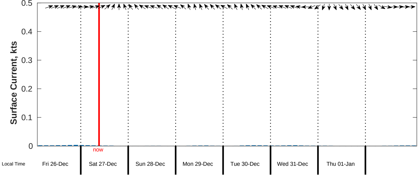
Surface Current Forecast for CSA (ONHYM) PPL EBS - Mauritania from 26-Dec-2025 00:00:00 to 03-Jan-2026 00:00:00
