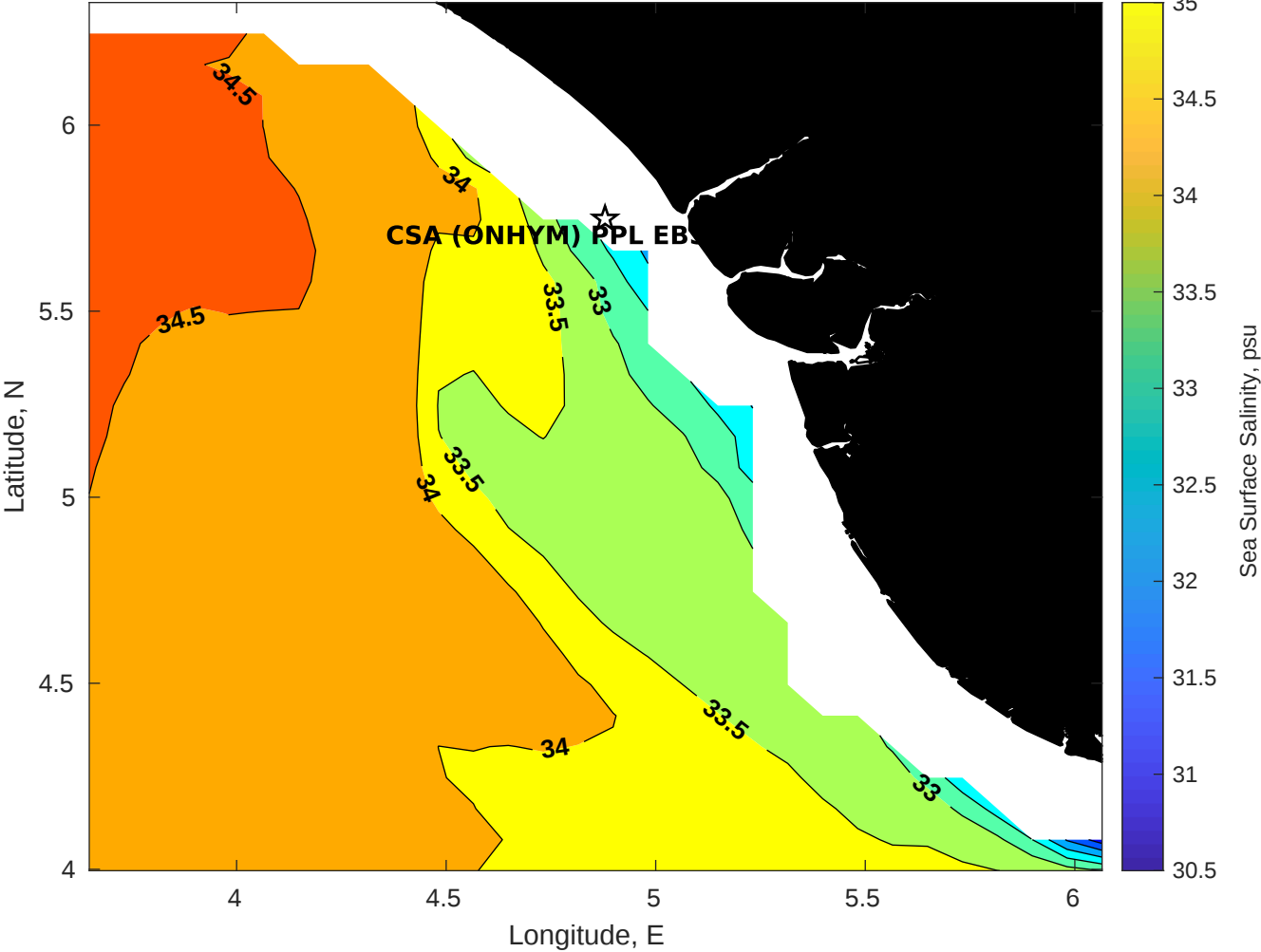
Surface Salinity for CSA (ONHYM) PPL EBS - Nigeria at 26-Dec-2025 00:00:00
