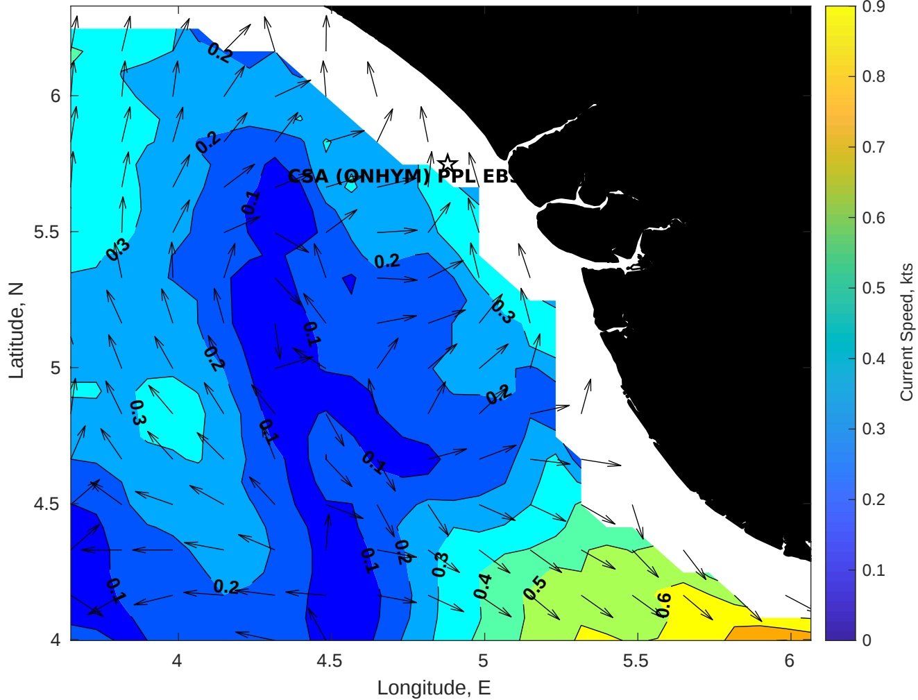
Surface Currents for CSA (ONHYM) PPL EBS - Nigeria at 26-Dec-2025 00:00:00
