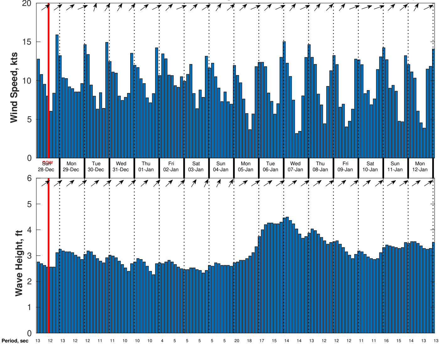
Wind & Wave Forecast for CSA (ONHYM) PPL EBS - Nigeria from 27-Dec-2025 02:00:00 to 12-Jan-2026 02:00:00
