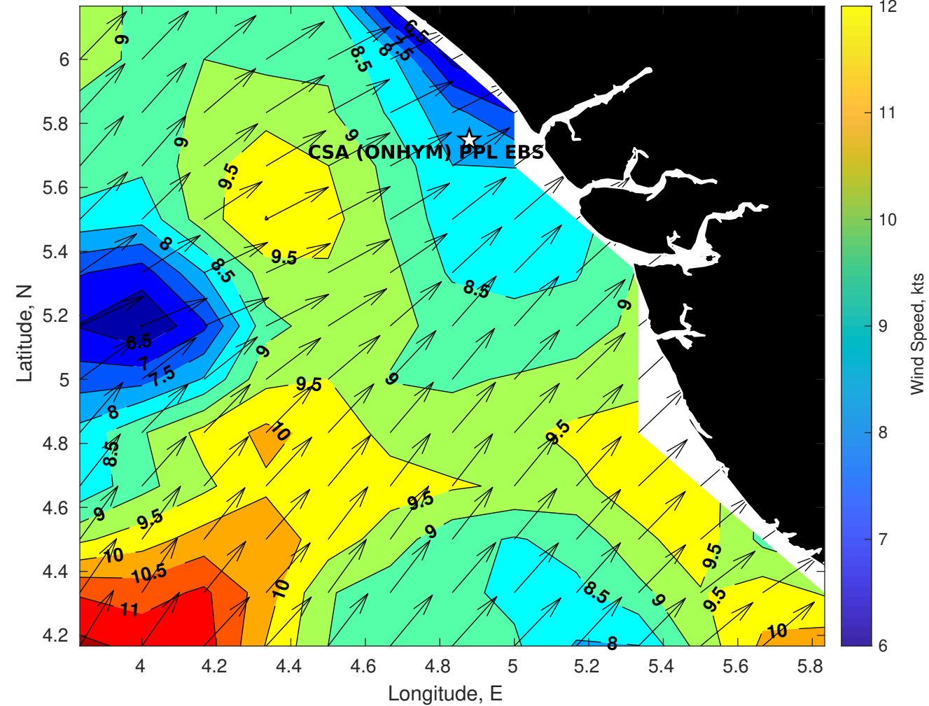
GFS Winds (kts) for CSA (ONHYM) PPL EBS - Nigeria at 27-Dec-2025 09:00:00
