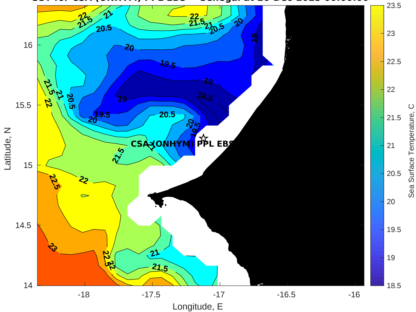
SST for CSA (ONHYM) PPL EBS - Senegal at 26-Dec-2025 00:00:00
