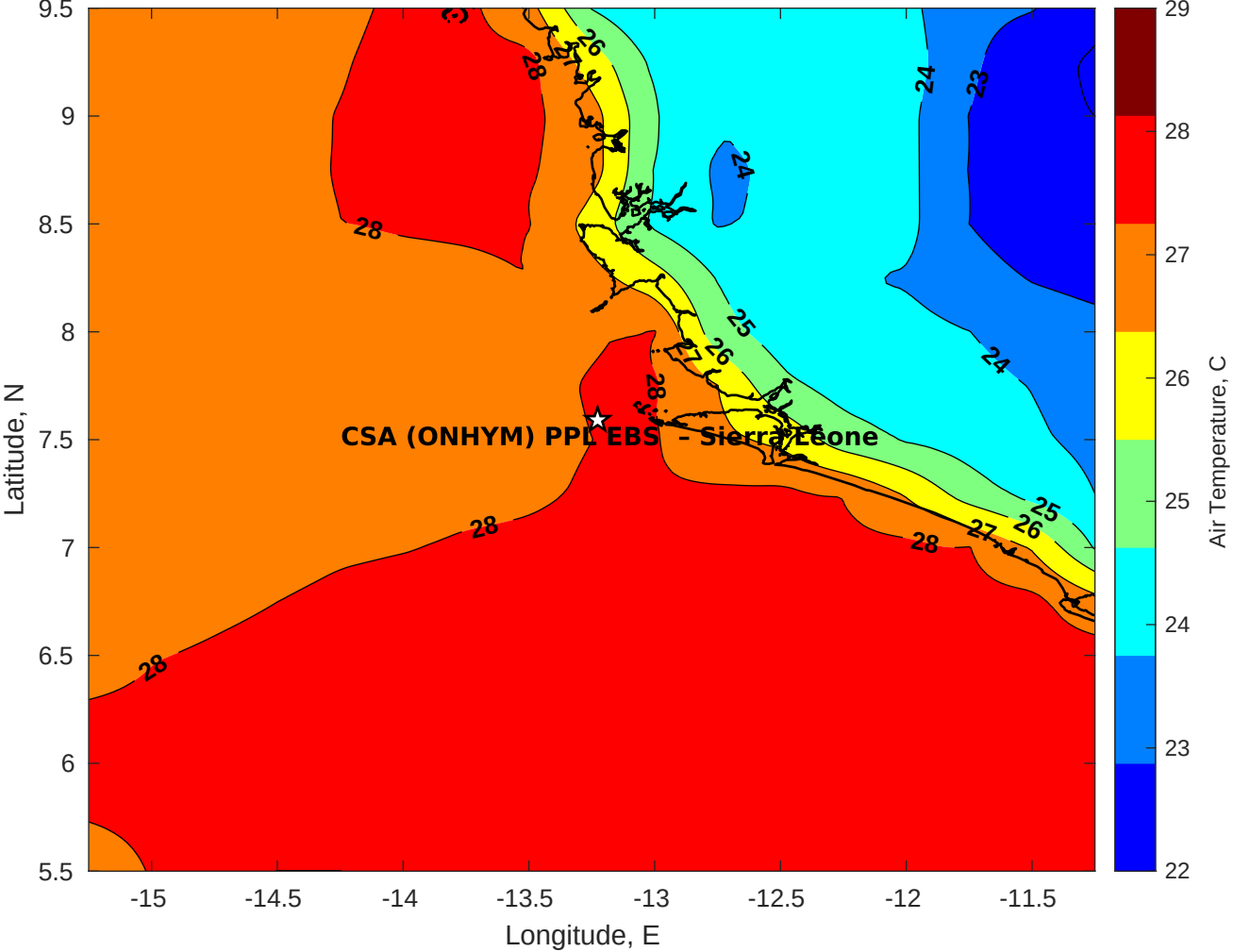
Air Temperature (C) for CSA (ONHYM) PPL EBS - Sierra Leone at 27-Dec-2025
