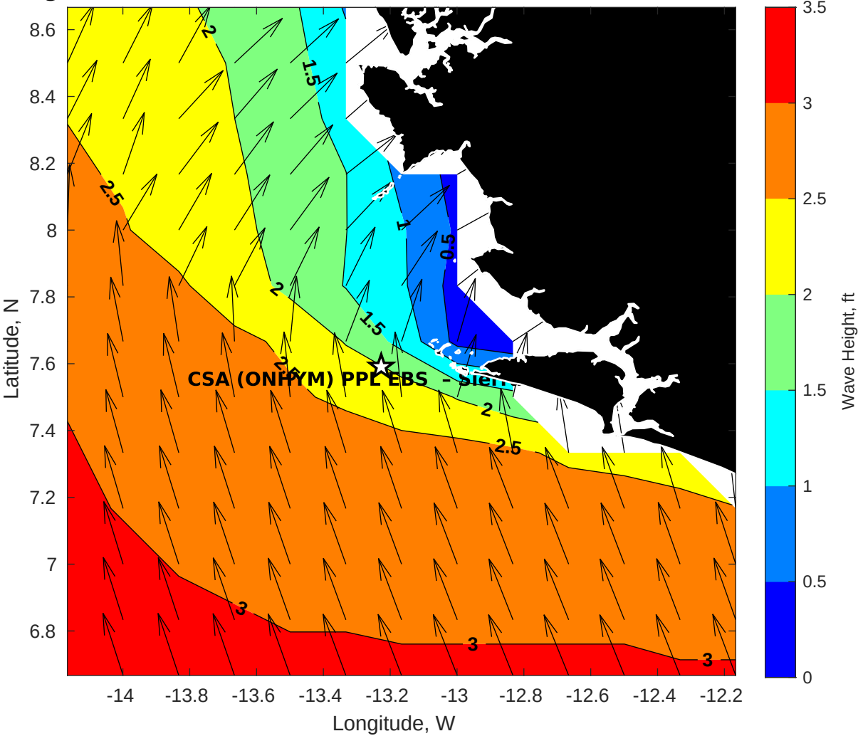
GFS Wave Height (ft) for CSA (ONHYM) PPL EBS - Sierra Leone at 27-Dec-2025 09:00:00
