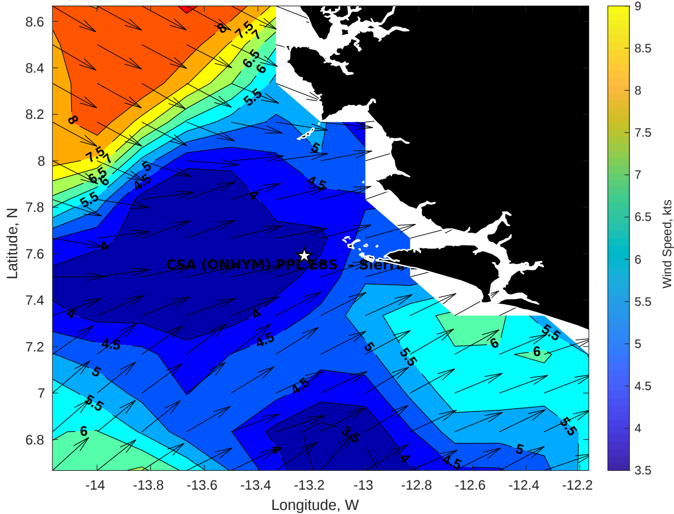
GFS Winds (kts) for CSA (ONHYM) PPL EBS - Sierra Leone at 27-Dec-2025 09:00:00
