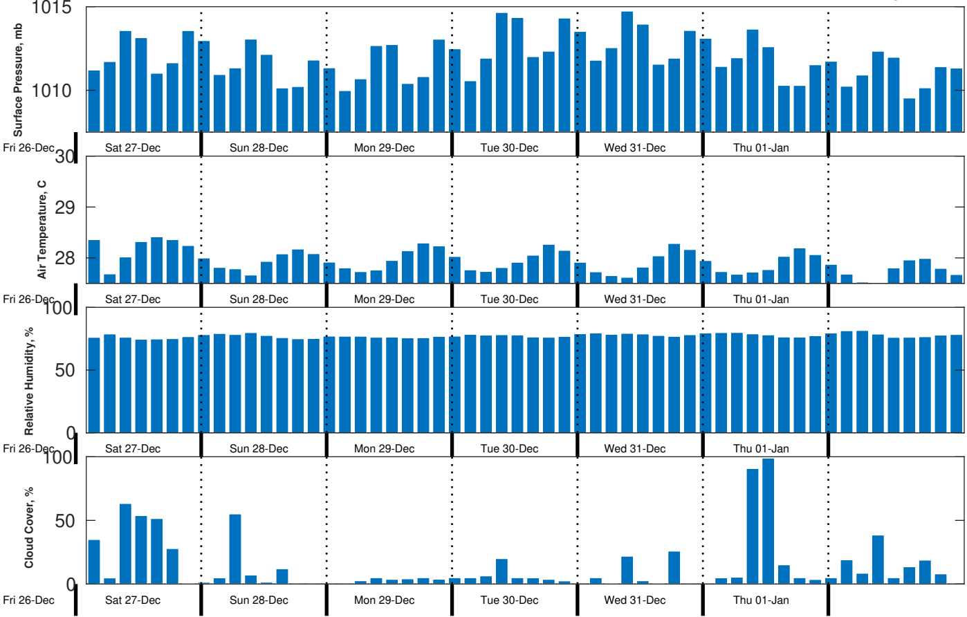
Met Forecast for CSA (ONHYM) PPL EBS - Sierra Leone from 27-Dec-2025 00:00:00 to 03-Jan-2026 00:00:00
