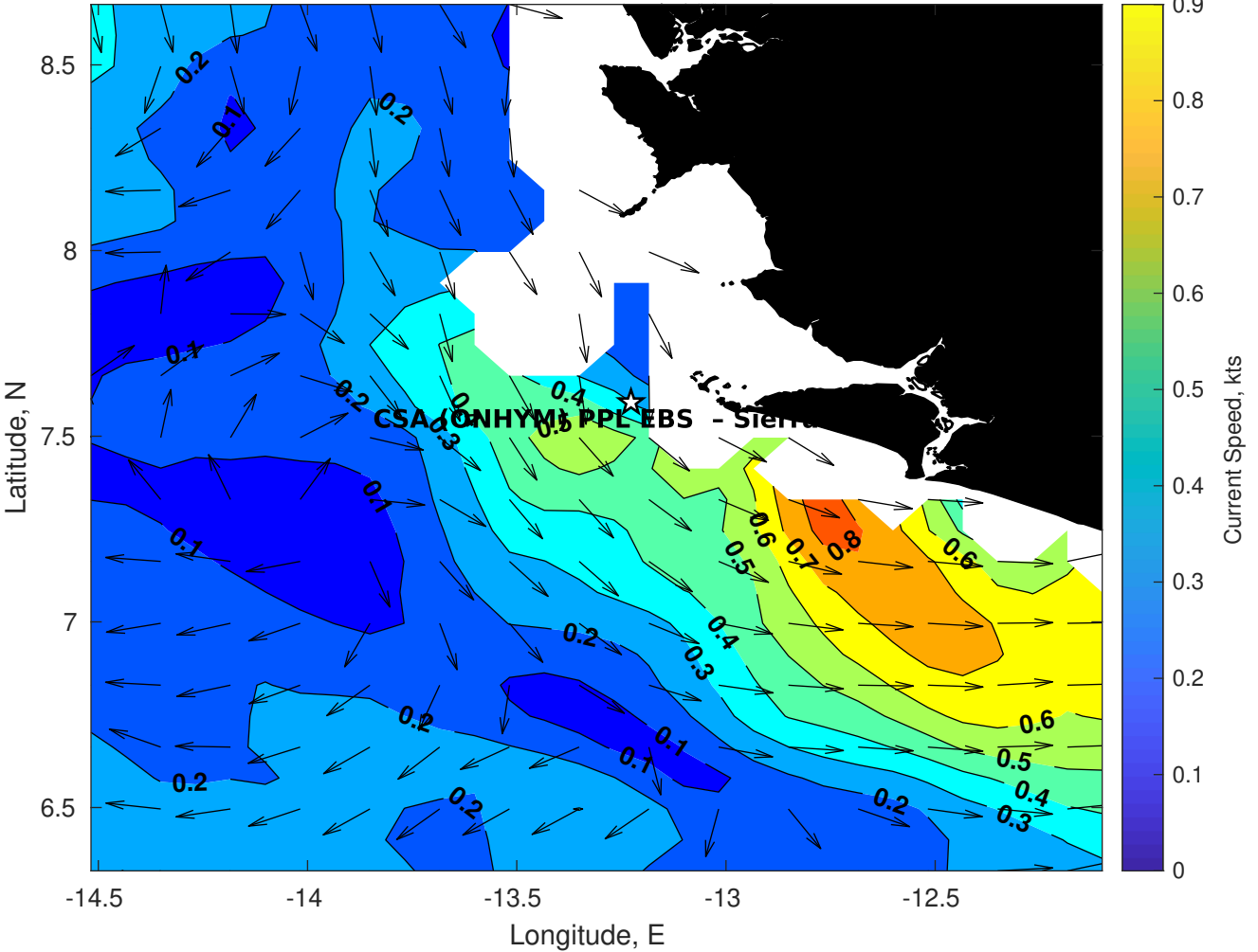
Surface Currents for CSA (ONHYM) PPL EBS - Sierra Leone at 26-Dec-2025 00:00:00
