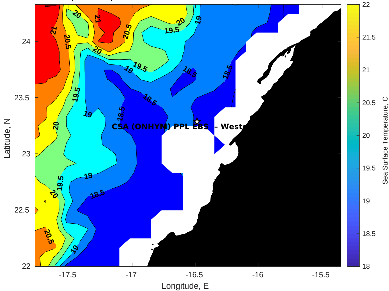
SST for CSA (ONHYM) PPL EBS - Western Sahara at 26-Dec-2025 00:00:00
