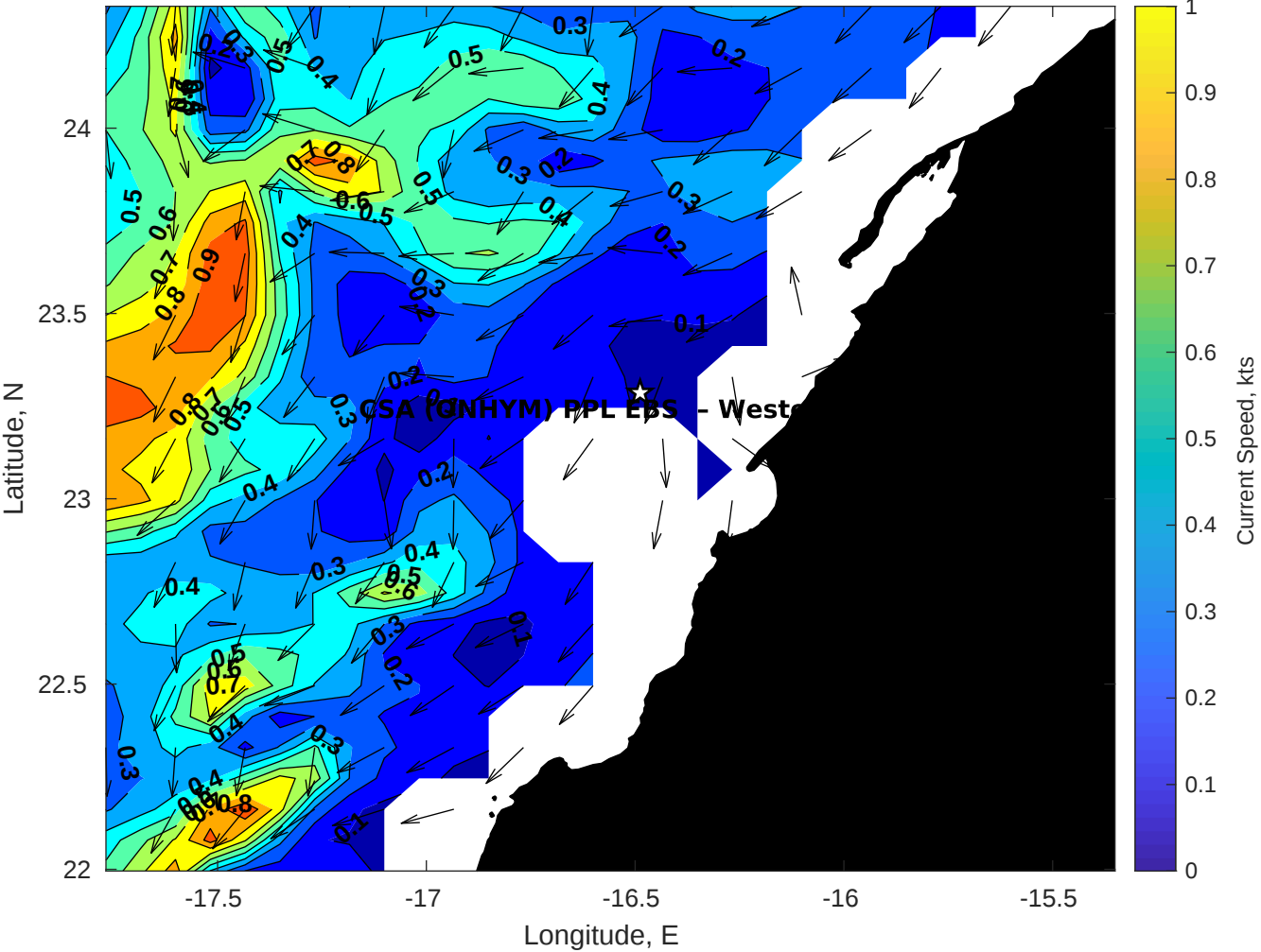
Surface Currents for CSA (ONHYM) PPL EBS - Western Sahara at 26-Dec-2025 00:00:00
