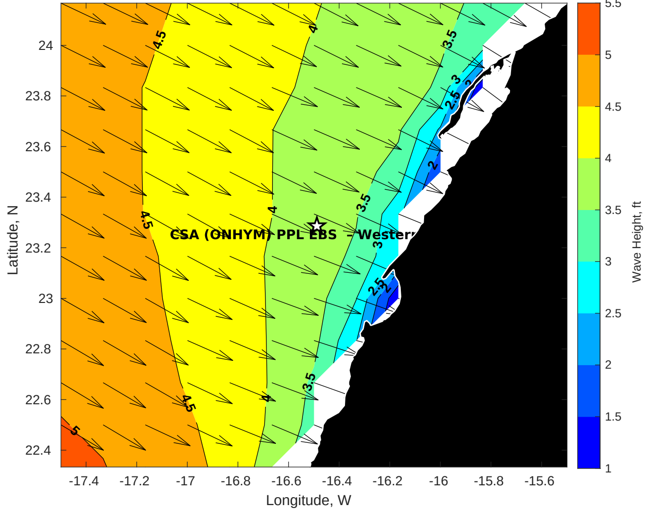
GFS Wave Height (ft) for CSA (ONHYM) PPL EBS - Western Sahara at 27-Dec-2025 09:00:00
