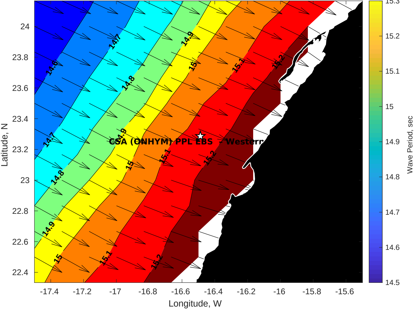
GFS Wave Period (sec) for CSA (ONHYM) PPL EBS - Western Sahara at 27-Dec-2025 09:00:00
