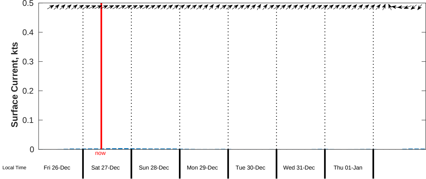
Surface Current Forecast for CSA (ONHYM) PPL EBS - Western Sahara from 26-Dec-2025 00:00:00 to 03-Jan-2026 00:00:00
