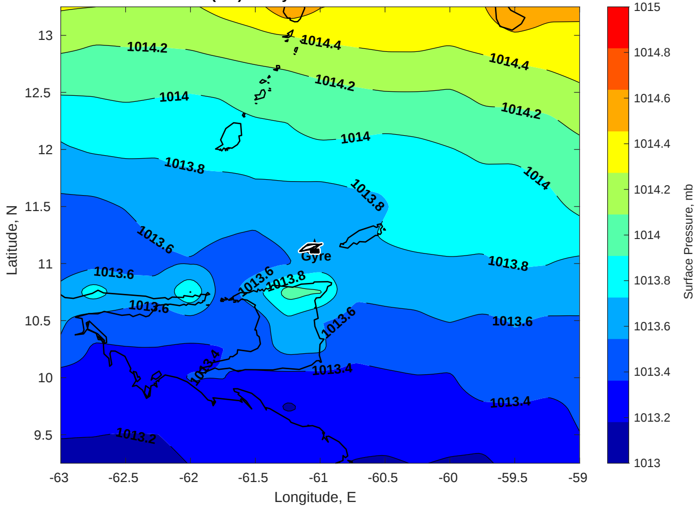
Surface Pressure (mb) for Gyre at 29-Dec-2025 00:00:00
