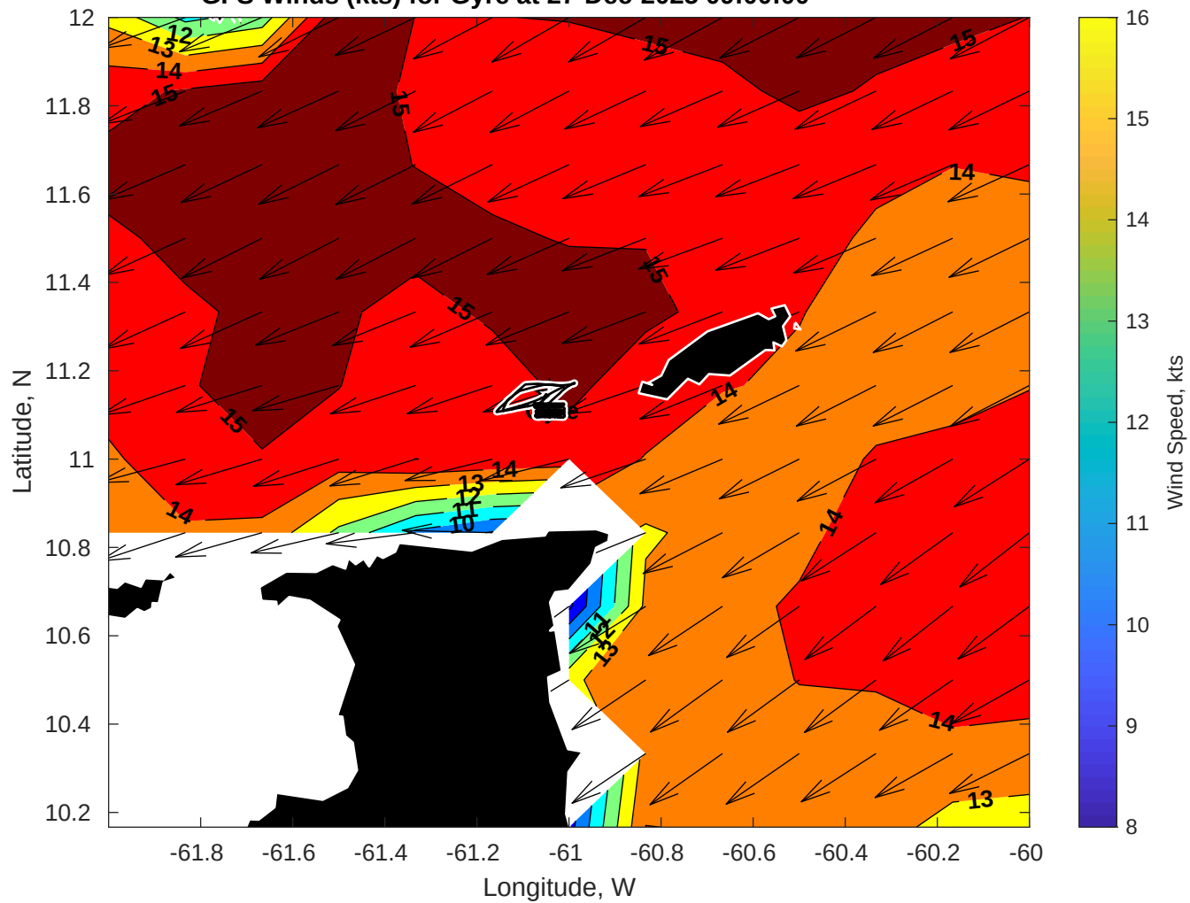
GFS Winds (kts) for Gyre at 27-Dec-2025 09:00:00
