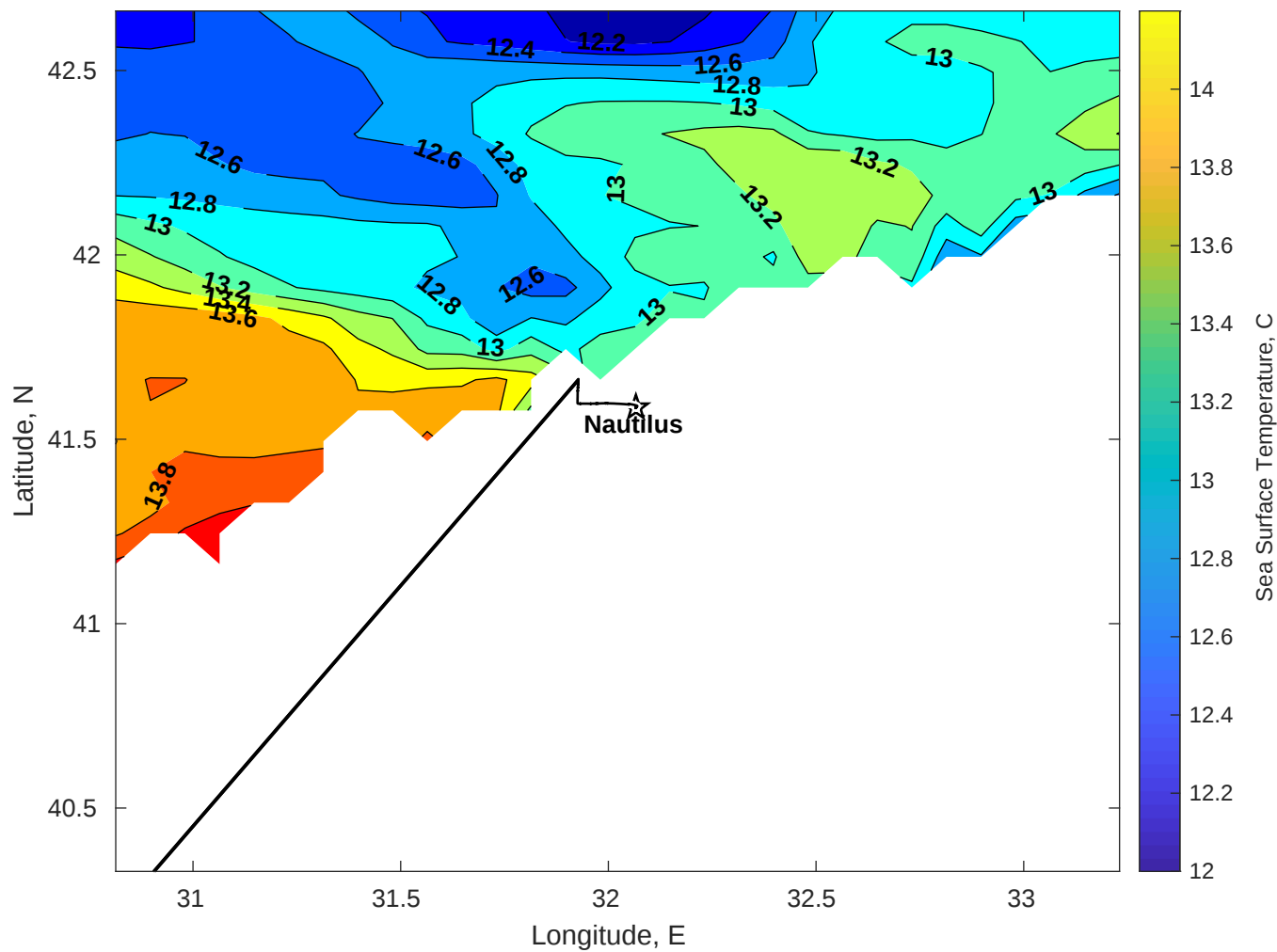
SST for Nautilus at 26-Dec-2025 00:00:00
