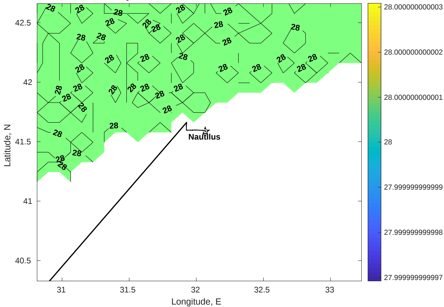
Surface Salinity for Nautilus at 26-Dec-2025 00:00:00
