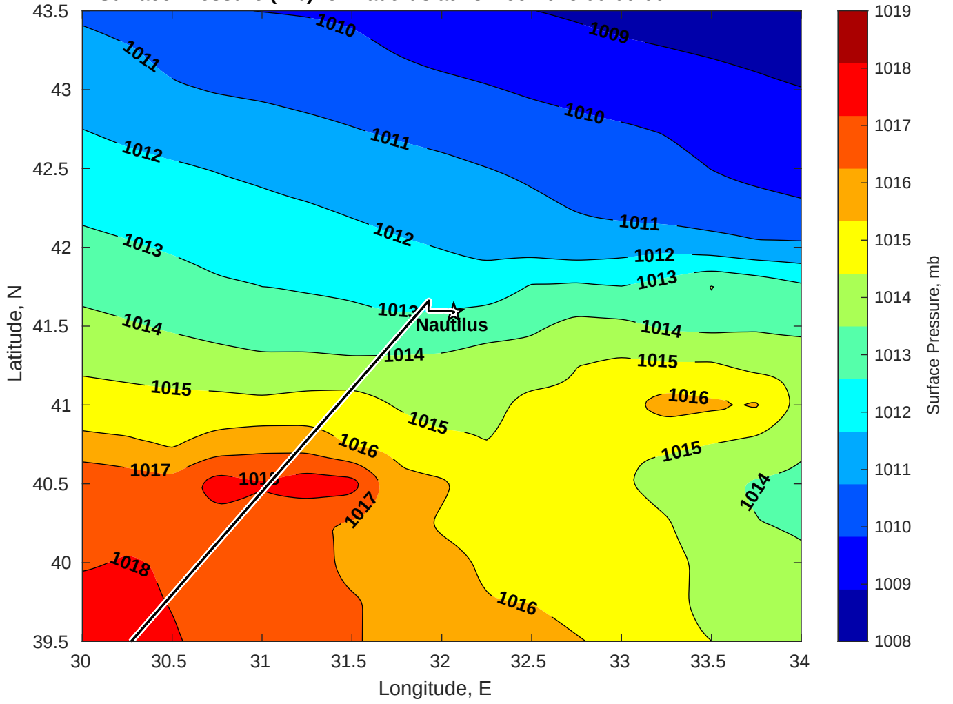
Surface Pressure (mb) for Nautilus at 28-Dec-2025 00:00:00
