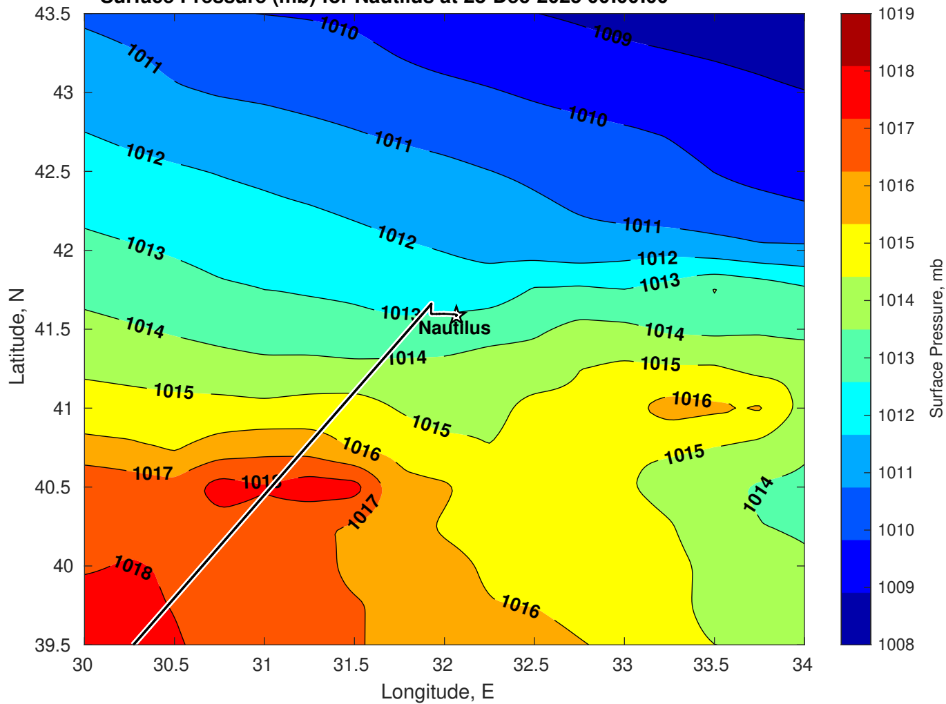
Surface Pressure (mb) for Nautilus at 28-Dec-2025 00:00:00
