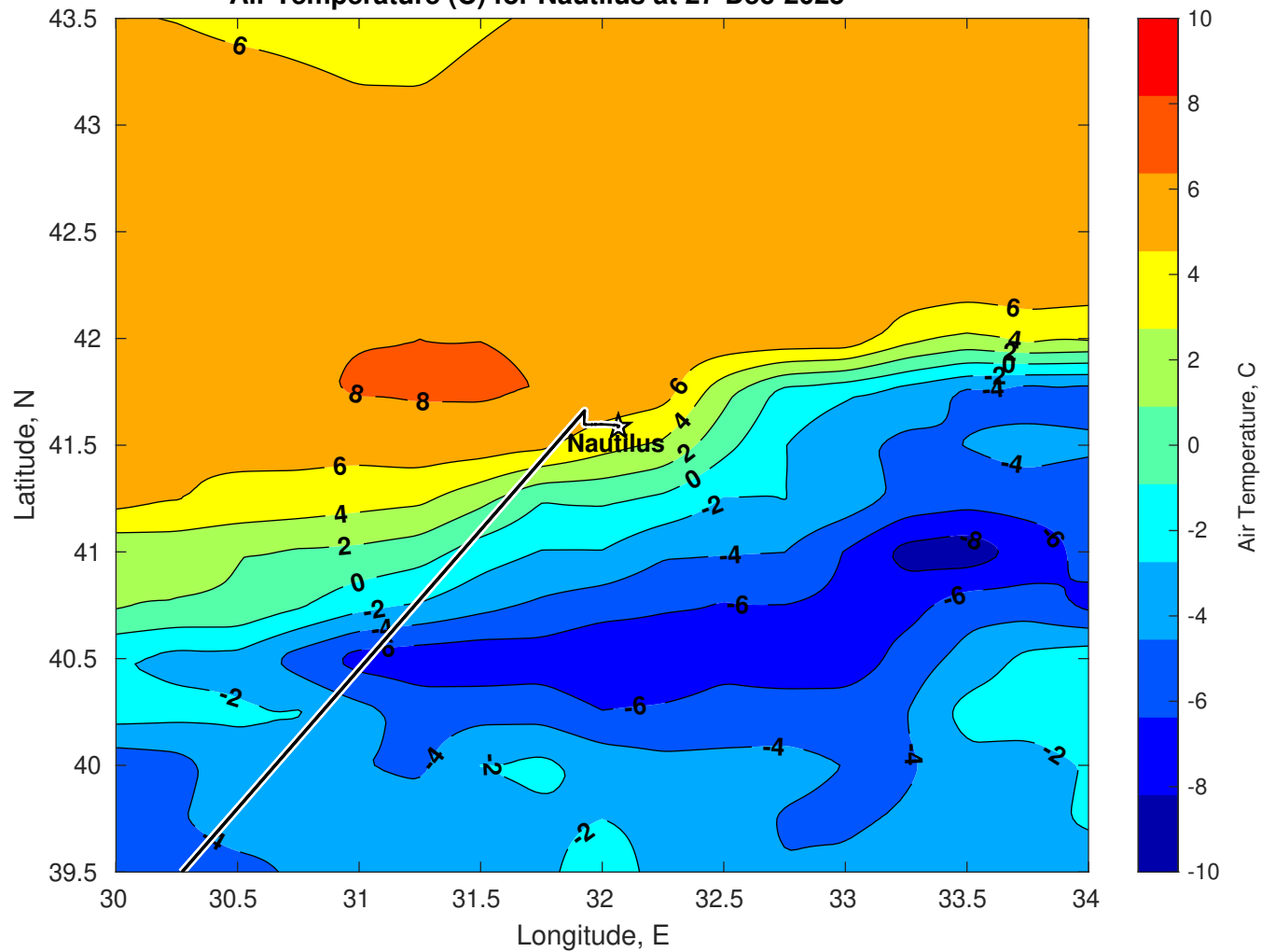
Air Temperature (C) for Nautilus at 27-Dec-2025
