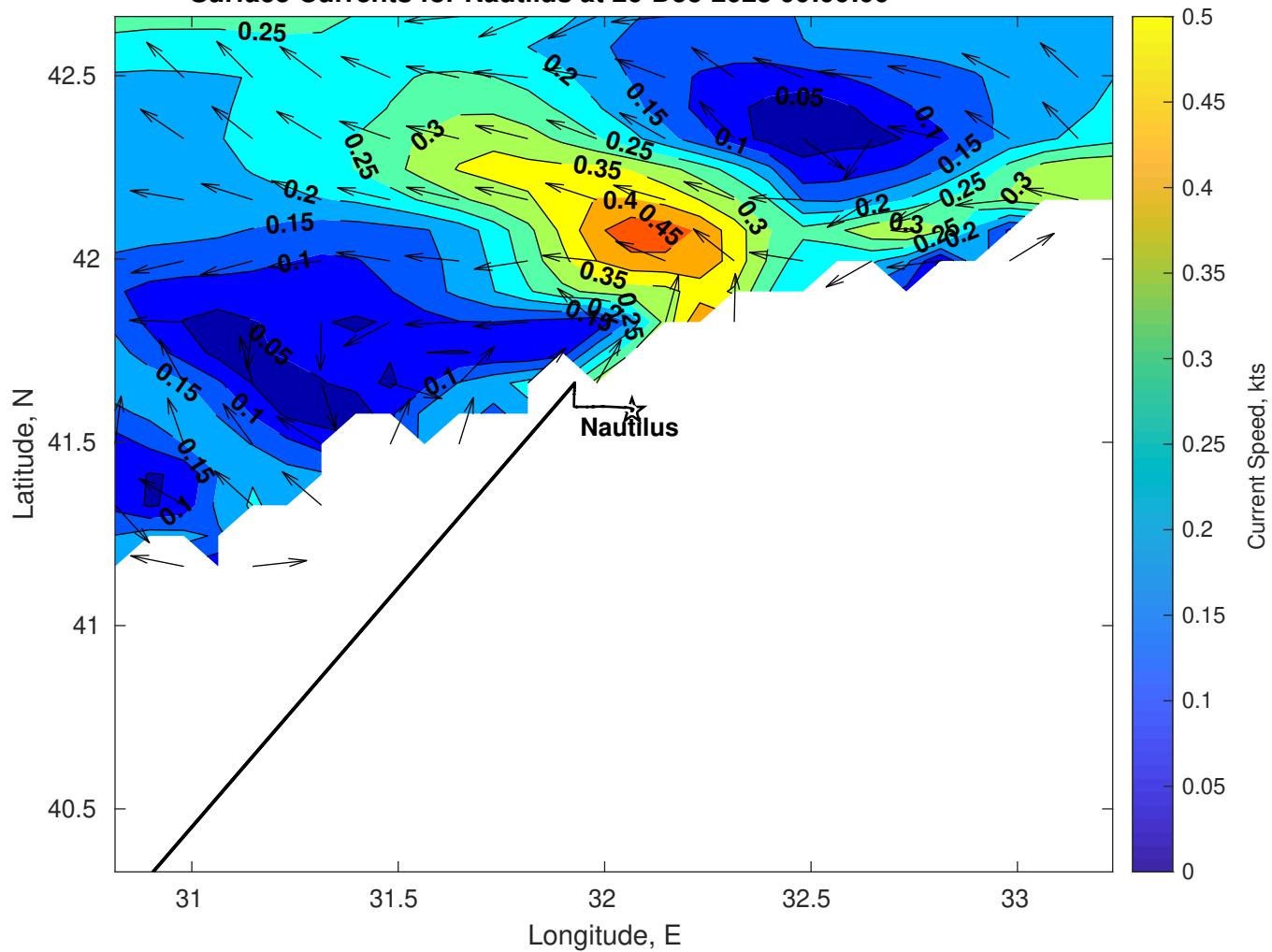
Surface Currents for Nautilus at 26-Dec-2025 00:00:00
