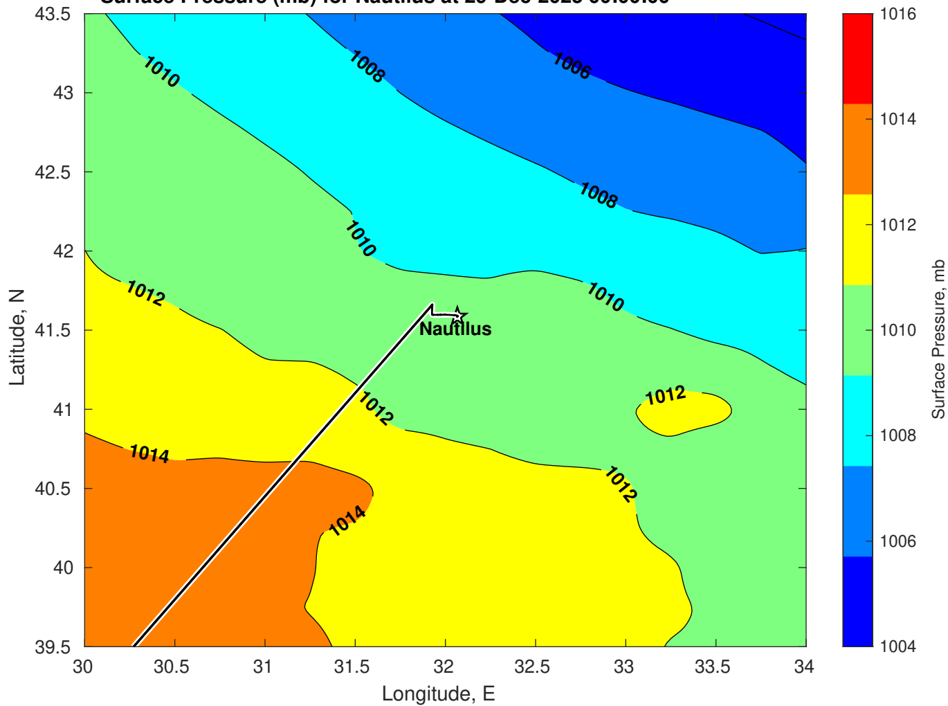
Surface Pressure (mb) for Nautilus at 29-Dec-2025 00:00:00
