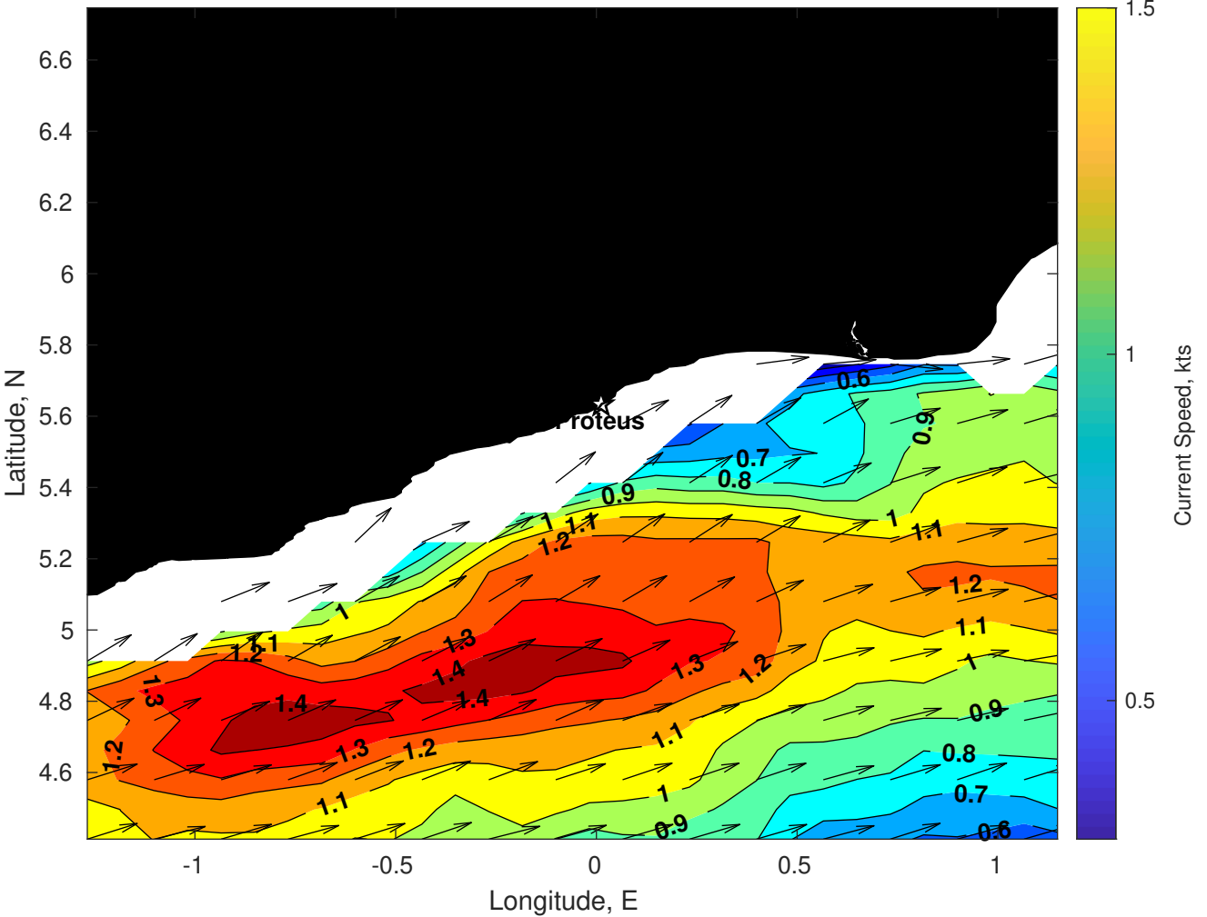
Surface Currents for Proteus at 26-Dec-2025 00:00:00
