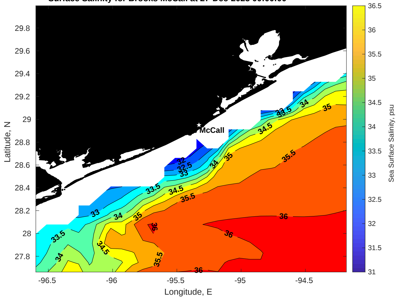
Surface Salinity for Brooks McCall at 27-Dec-2025 00:00:00
