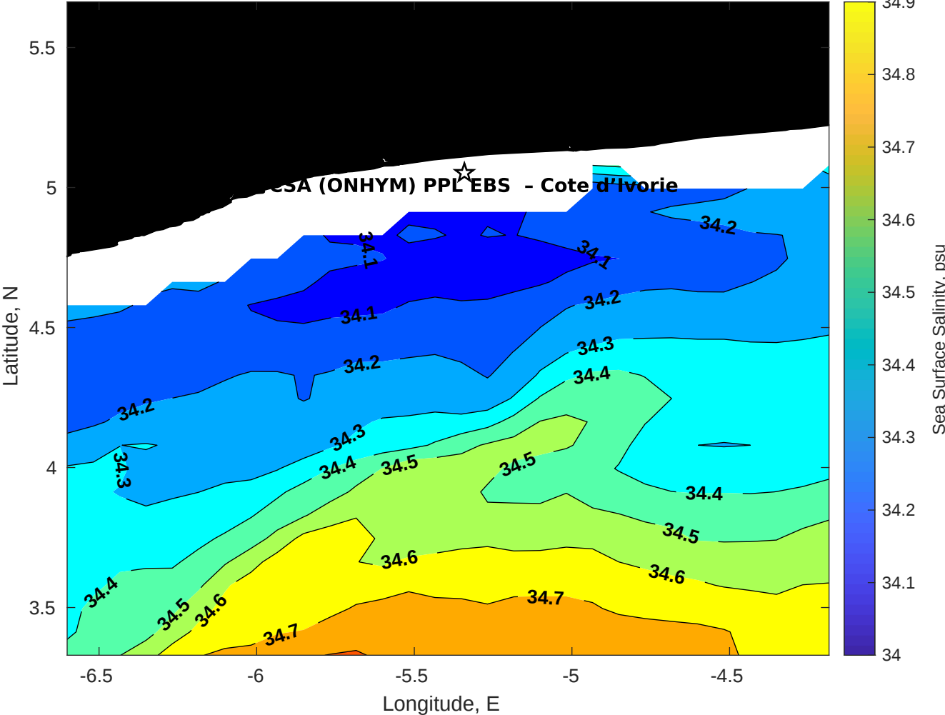
Surface Salinity for CSA (ONHYM) PPL EBS - Cote d'Ivoire at 27-Dec-2025 00:00:00
