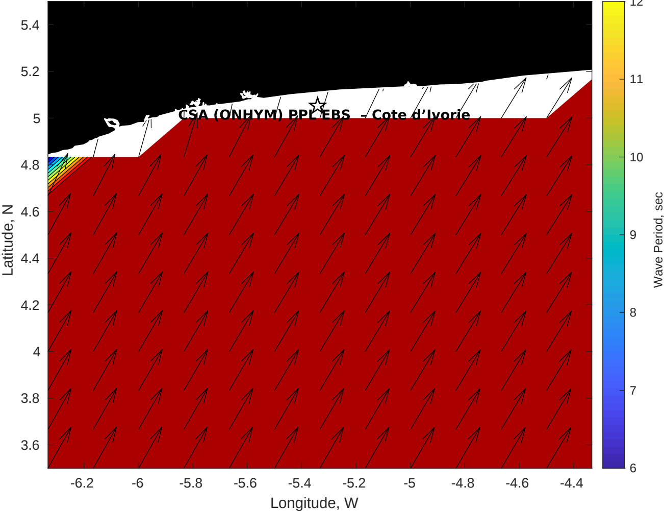
GFS Wave Period (sec) for CSA (ONHYM) PPL EBS - Cote d'Ivoire at 28-Dec-2025 09:00:00
