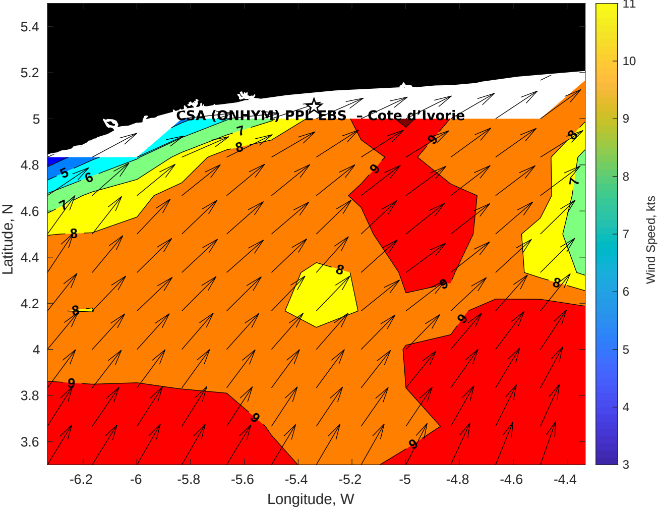
GFS Winds (kts) for CSA (ONHYM) PPL EBS - Cote d'Ivoire at 28-Dec-2025 09:00:00
