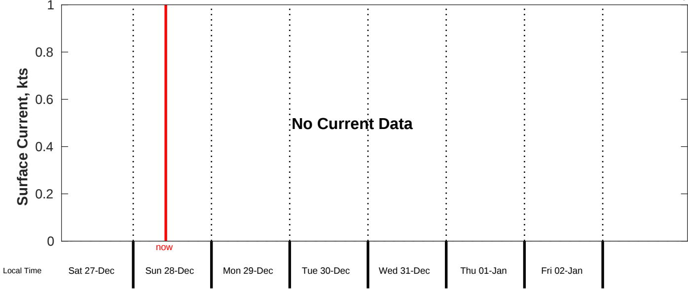
Surface Current Forecast for CSA (ONHYM) PPL EBS - Cote d'Ivoire from 27-Dec-2025 00:00:00 to 04-Jan-2026 00:00:00
