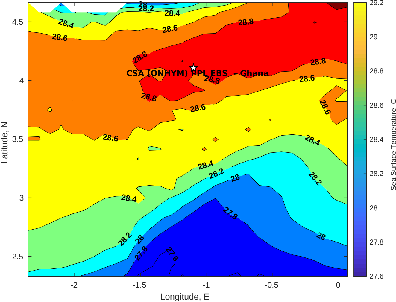
SST for CSA (ONHYM) PPL EBS - Ghana at 27-Dec-2025 00:00:00
