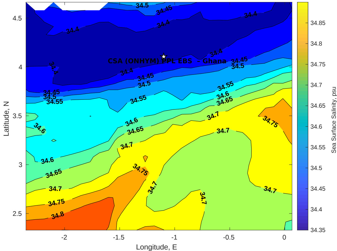
Surface Salinity for CSA (ONHYM) PPL EBS - Ghana at 27-Dec-2025 00:00:00
