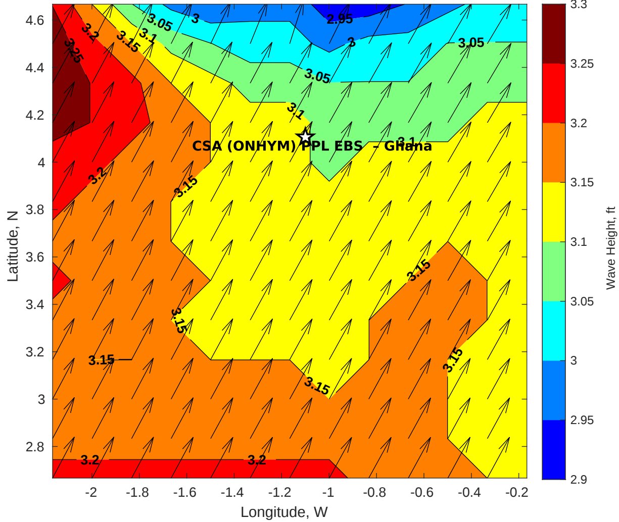
GFS Wave Height (ft) for CSA (ONHYM) PPL EBS - Ghana at 28-Dec-2025 09:00:00
