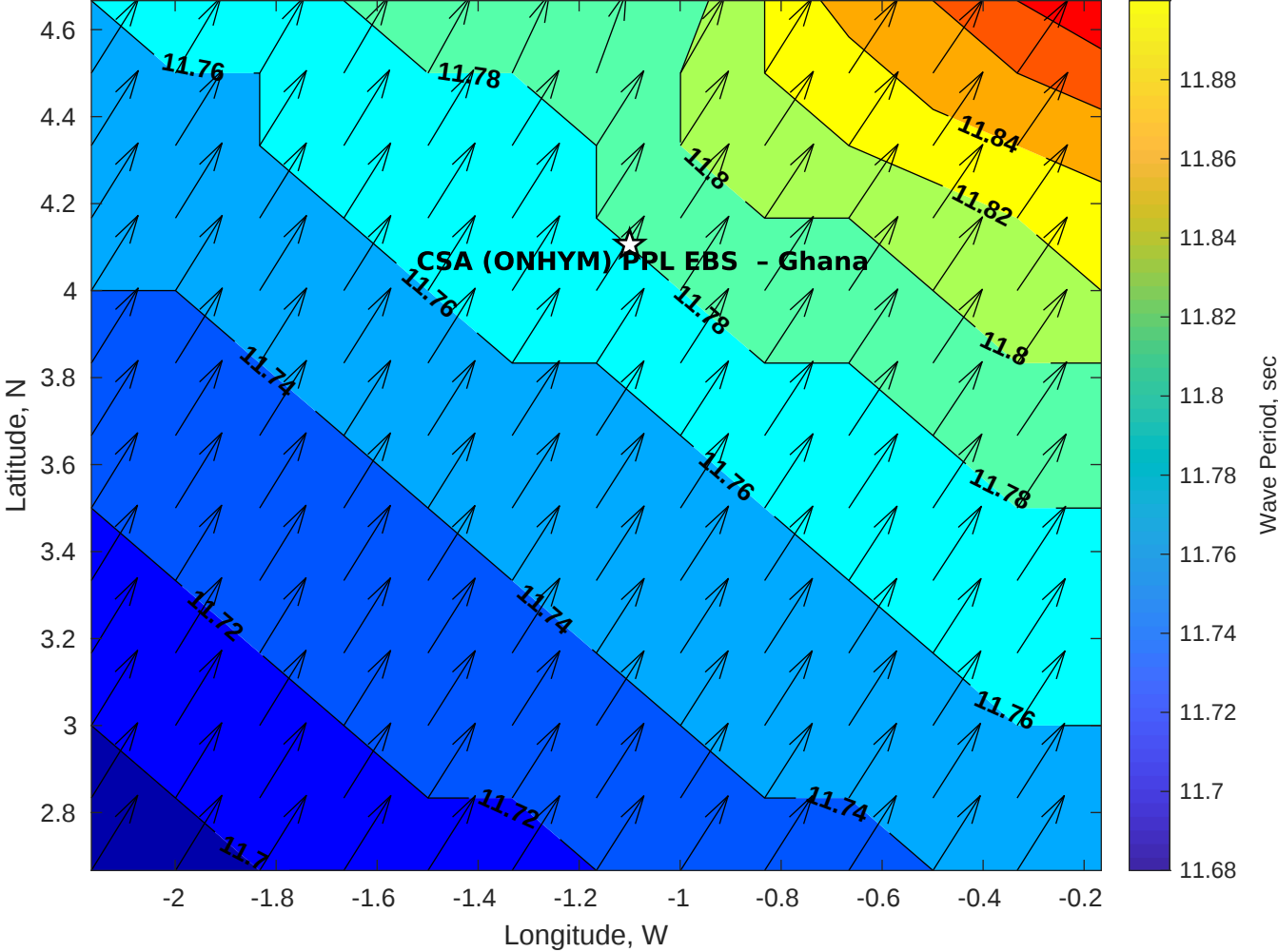
GFS Wave Period (sec) for CSA (ONHYM) PPL EBS - Ghana at 28-Dec-2025 09:00:00
