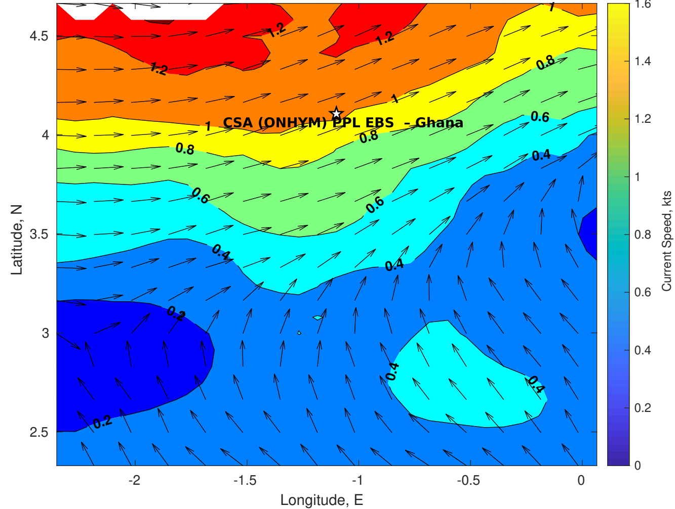
Surface Currents for CSA (ONHYM) PPL EBS - Ghana at 27-Dec-2025 00:00:00
