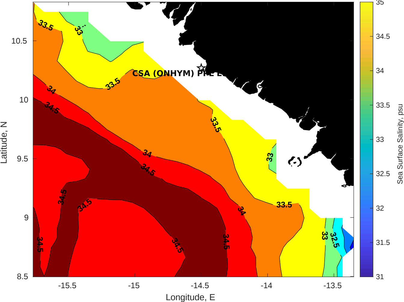
Surface Salinity for CSA (ONHYM) PPL EBS - Guinea at 27-Dec-2025 00:00:00
