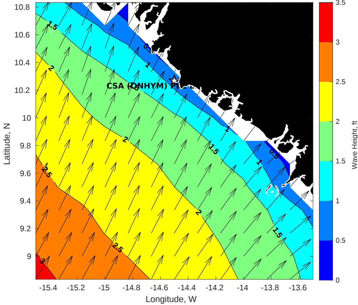
GFS Wave Height (ft) for CSA (ONHYM) PPL EBS - Guinea at 28-Dec-2025 09:00:00
