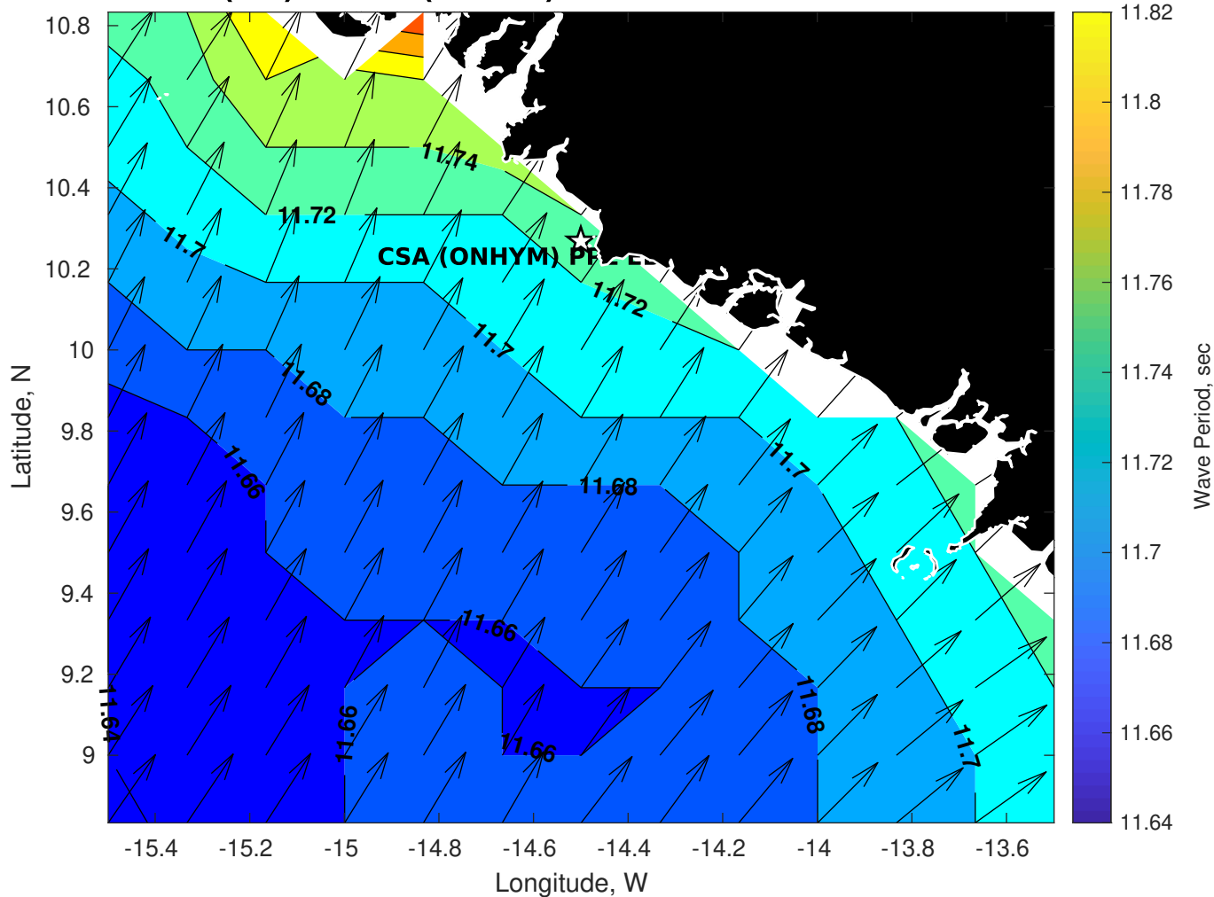
GFS Wave Period (sec) for CSA (ONHYM) PPL EBS - Guinea at 28-Dec-2025 09:00:00
