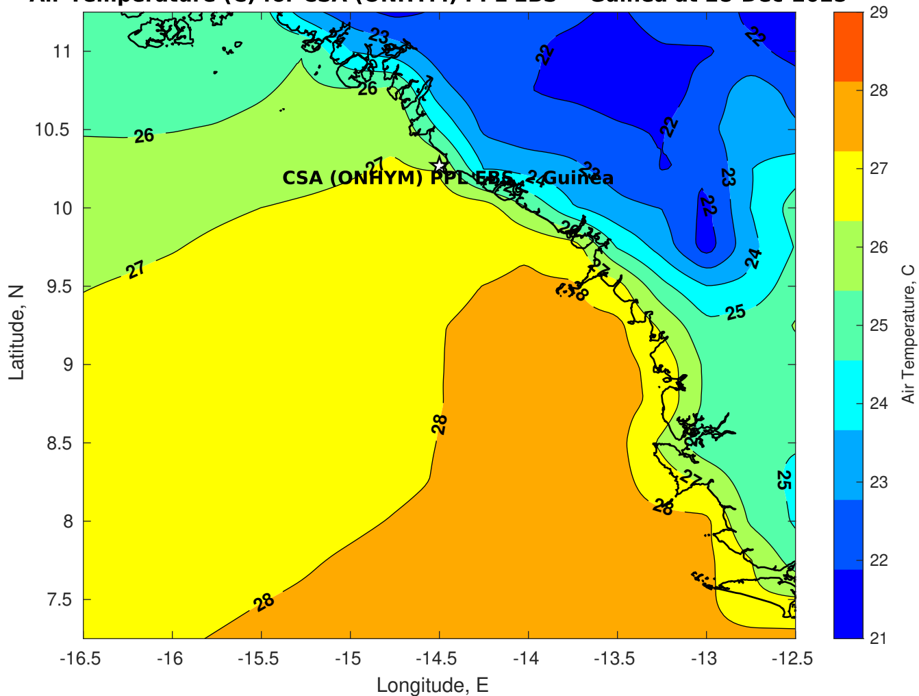
Air Temperature (C) for CSA (ONHYM) PPL EBS - Guinea at 28-Dec-2025
