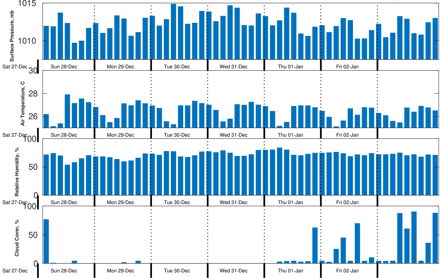
Met Forecast for CSA (ONHYM) PPL EBS - Guinea from 28-Dec-2025 00:00:00 to 04-Jan-2026 00:00:00
