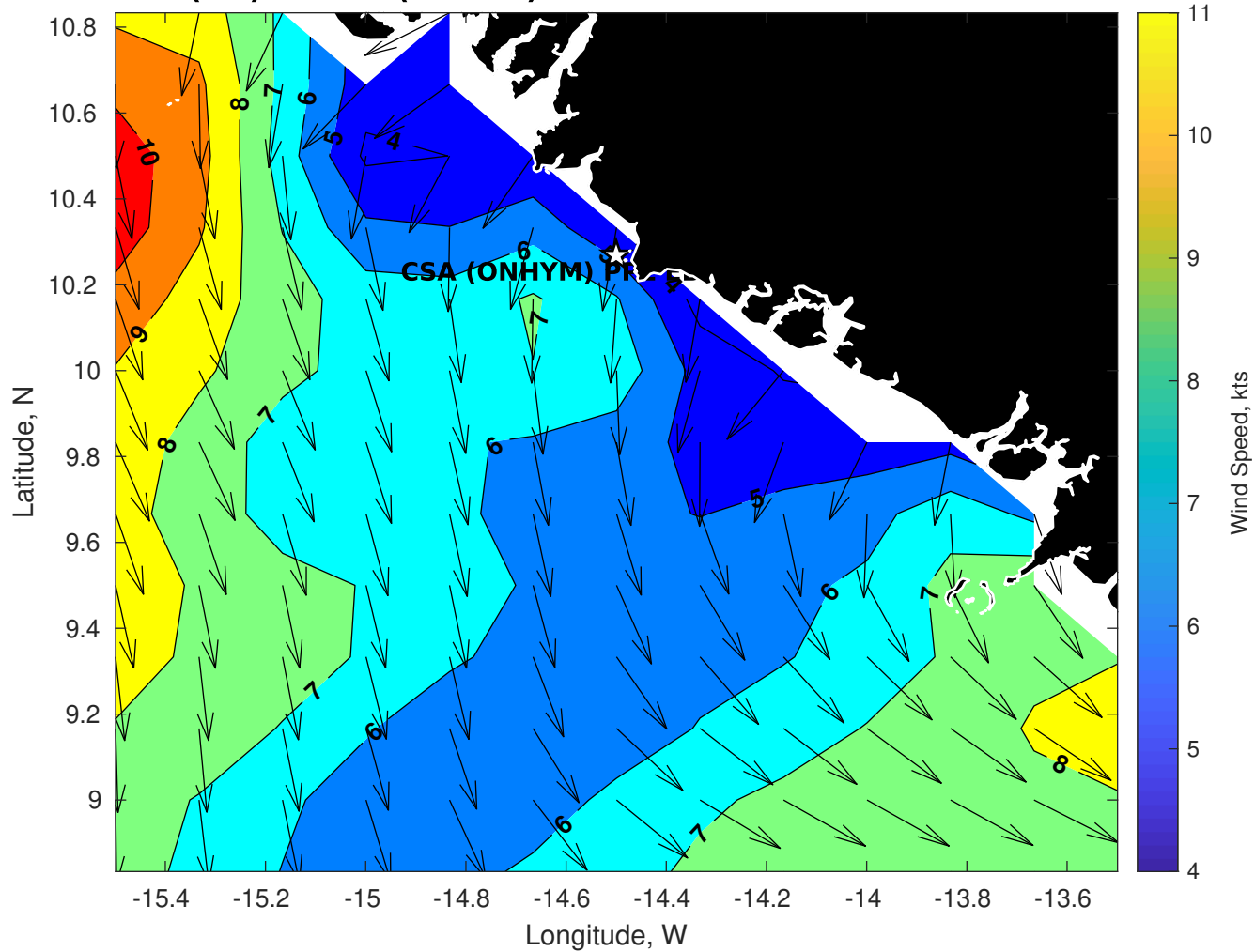
GFS Winds (kts) for CSA (ONHYM) PPL EBS - Guinea at 28-Dec-2025 09:00:00
