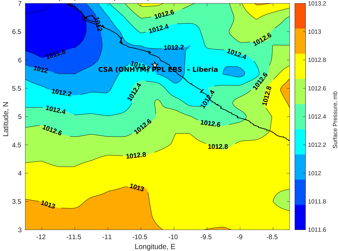
Surface Pressure (mb) for CSA (ONHYM) PPL EBS - Liberia at 29-Dec-2025 00:00:00
