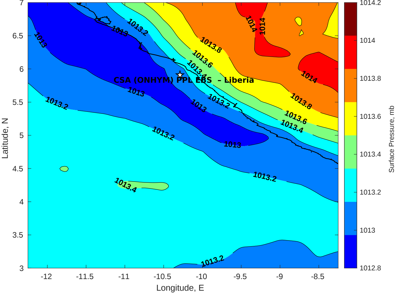
Surface Pressure (mb) for CSA (ONHYM) PPL EBS - Liberia at 30-Dec-2025 00:00:00
