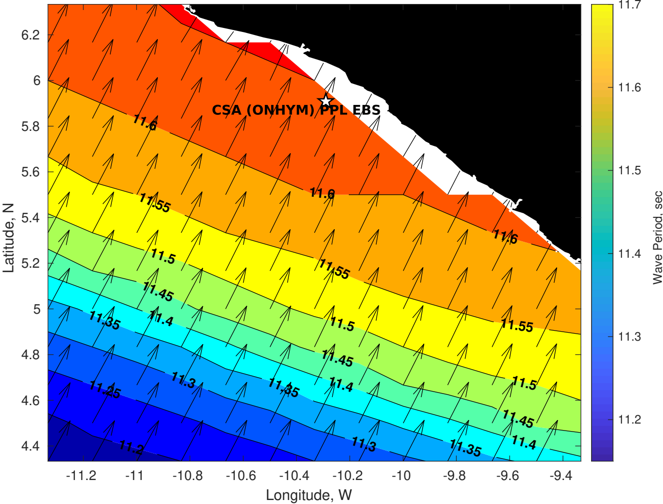
GFS Wave Period (sec) for CSA (ONHYM) PPL EBS - Liberia at 28-Dec-2025 09:00:00
