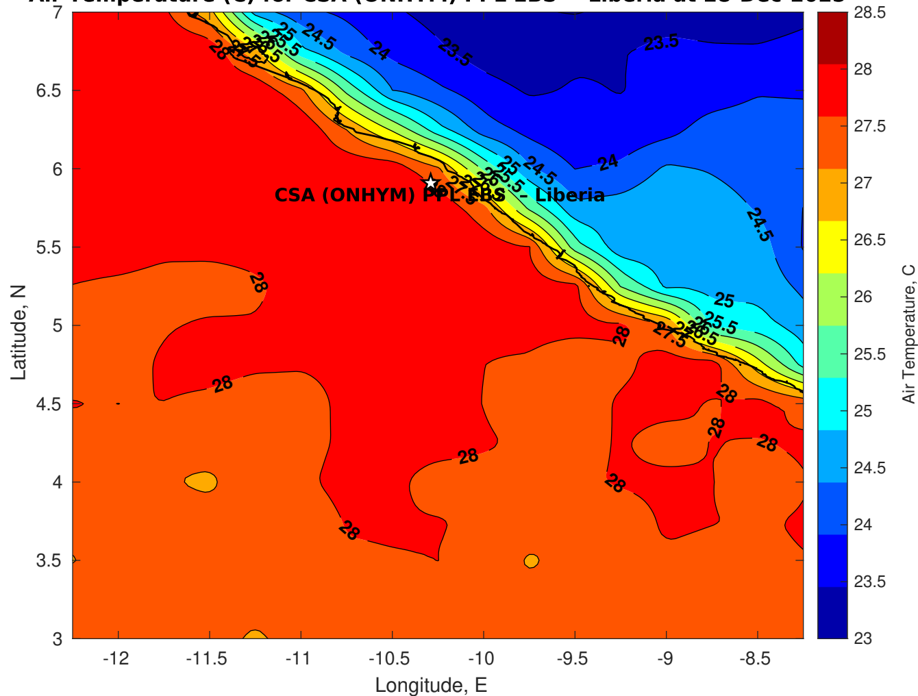
Air Temperature (C) for CSA (ONHYM) PPL EBS - Liberia at 28-Dec-2025
