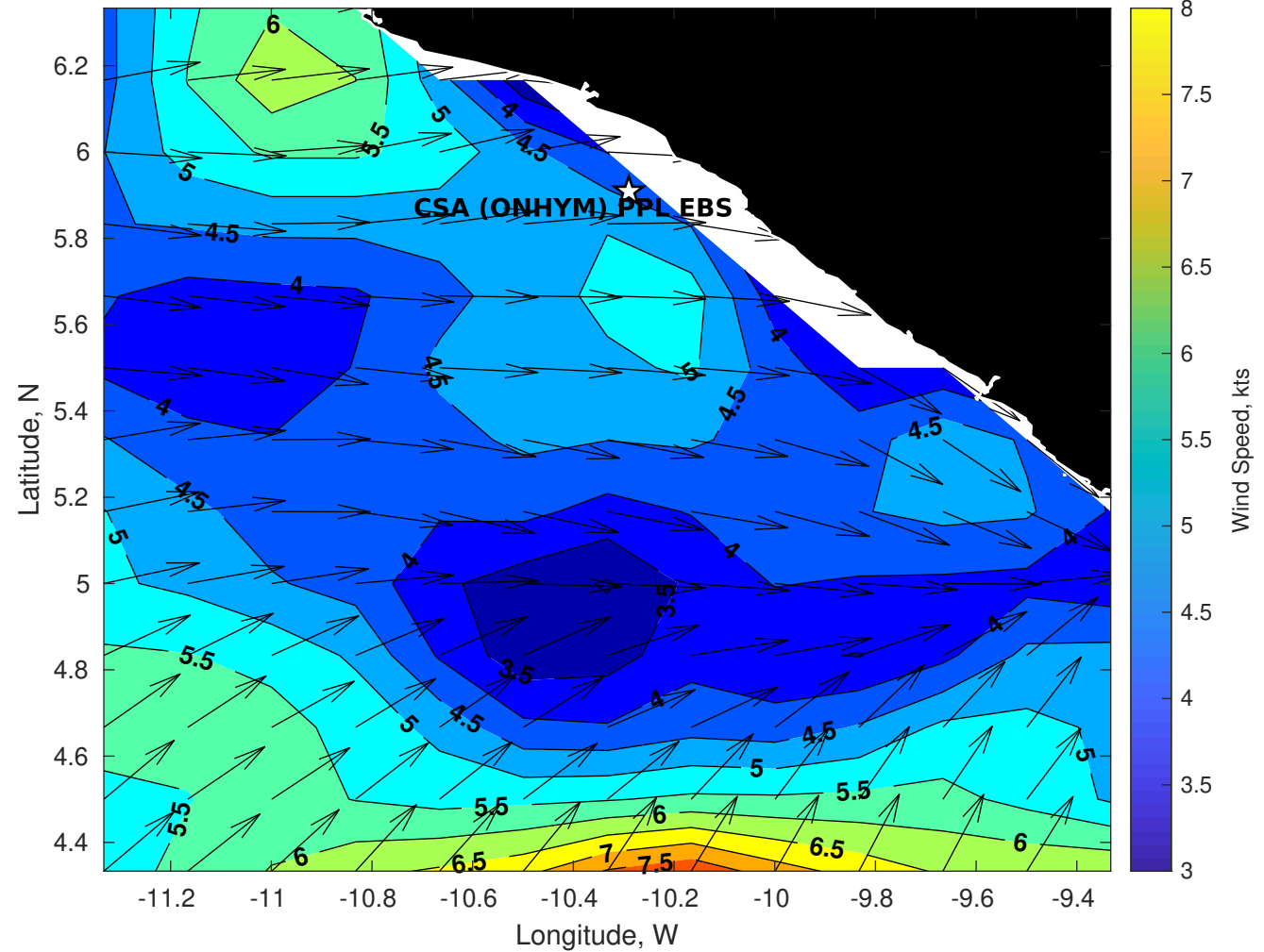
GFS Winds (kts) for CSA (ONHYM) PPL EBS - Liberia at 28-Dec-2025 09:00:00
