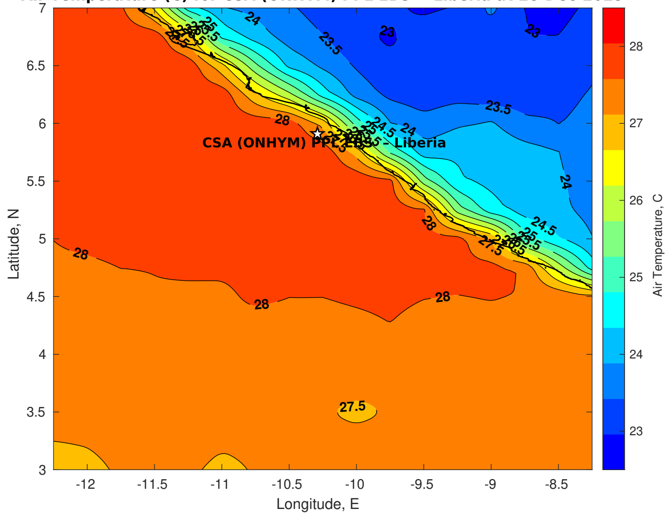
Air Temperature (C) for CSA (ONHYM) PPL EBS - Liberia at 28-Dec-2025
